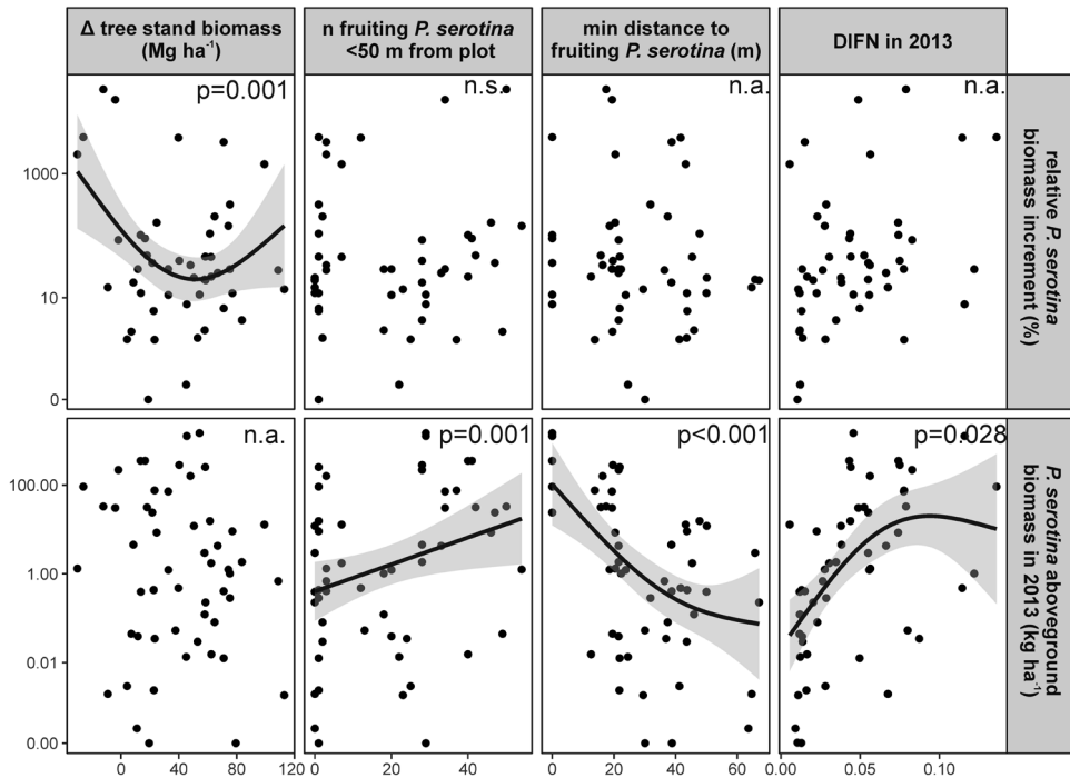
Figure 4. Responses of percentage increment of Prunus serotina biomass and total biomass in 2013 to the particular predictors. Lines were fitted using General Additive Models (see Table 1 for model parameters), grey area indicates SE of model, n.s. – not significant, n.a. – significance level not applicable as considered variable was not included in the final model (Table 1). Note the logarithmic scale of the Y axis.
