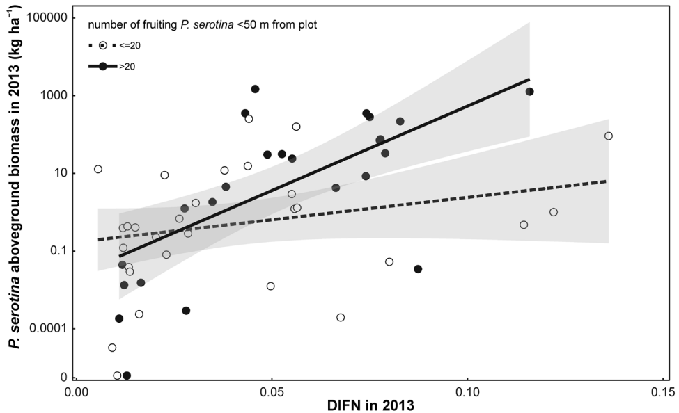
Figure 3. Relationship between light availability, expressed by DIFN, and aboveground biomass of P. serotina , in two classes of propagule pressure, expressed by the number of fruiting P. serotina trees up to 50 m from the plot (open dots and dashed line: \leq 20 ; solid dots and line: > 20 ; p < 0.001 , R^2 = 0.32 ). Threshold of 20 trees was chosen according to median and mean for all plots (18 and 18.49, respectively). Modification given by class of propagule pressure was statistically significant ( p < 0.01 ). Note log-transformation of the y axis. Shading around regression lines indicate range of model SE.
