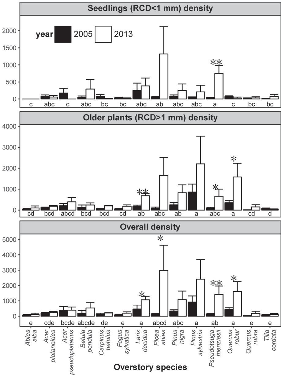
Figure 2. Mean +SE density (ind. ha -1 ) of Prunus serotina within experimental plots of 14 tree species in 2005 and in 2013. Asterisks mark significance levels of differences between inventories in 2005 and 2013 (* – p < 0.05 , ** – p < 0.01 ), based on Student's t-test. Letters under bars represent significance of differences among tree species in 2013, based on Kruskal-Wallis tests; there are no statistically significant differences between values marked by the same letter.
