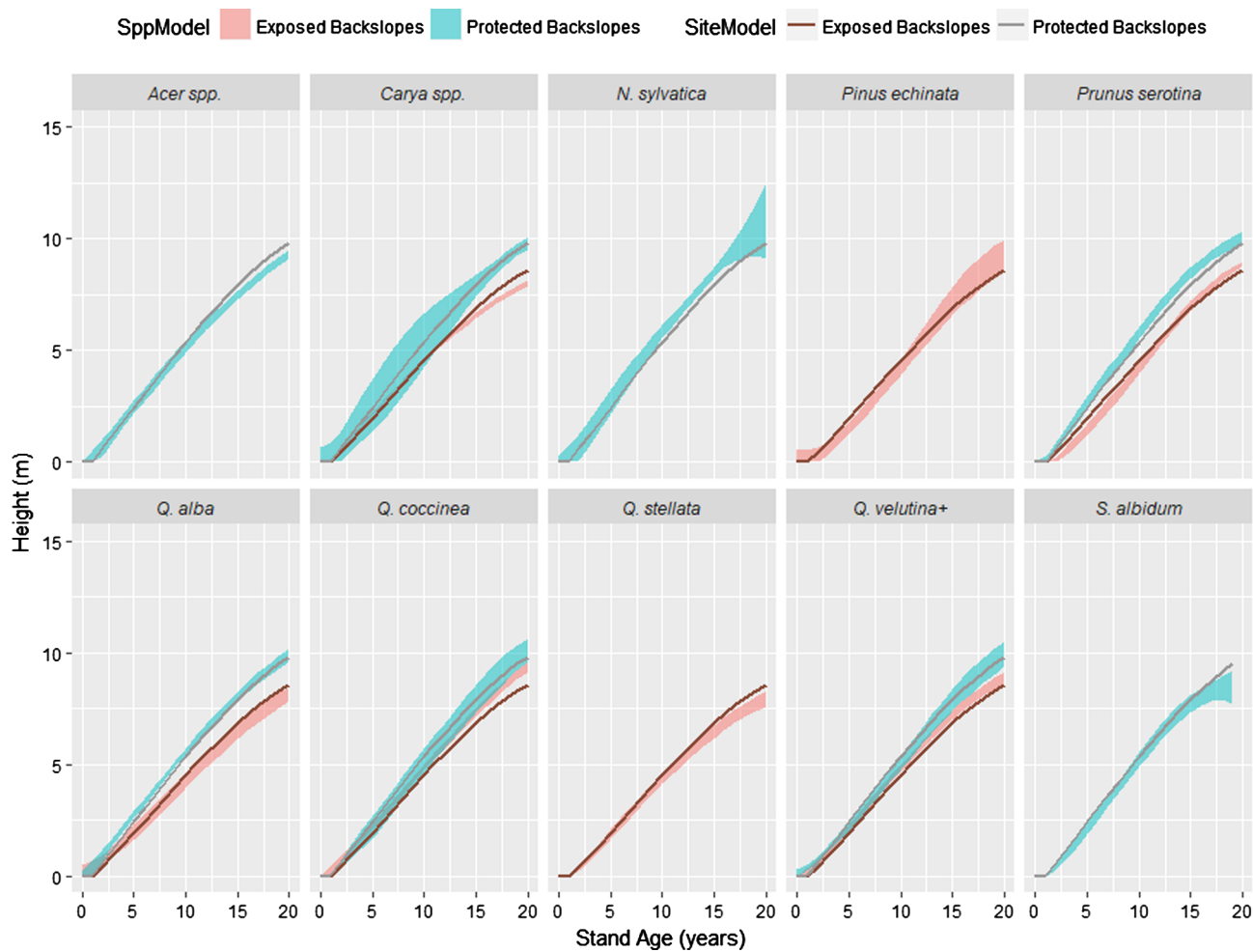
Fig. 4. Near-minima early height development by species and site class. Ribbons depict 95% confidence bands for quantile regression estimates (10th percentile) for species-specific models, lines depict quantile regression point estimates for models that are only site-specific (includes all species on a site class).
