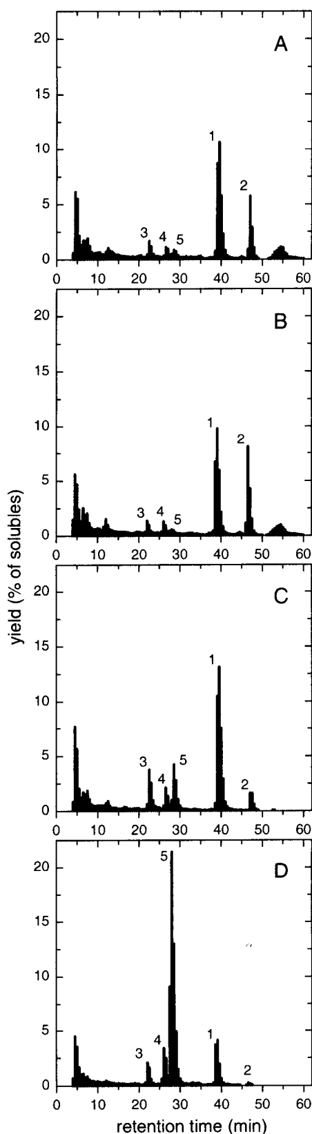
Fig. 2. HPLC radiochromatograms of products obtained from model 1 by peroxyl radical-generating systems. A: With MnP, Mn(II), and linoleic acid at 48 h. B: With H_2O_2 , Fe(II), and arachidonic acid at 144 h. C: With ACVA at 48 h. D: With AMPD at 3 h. Peaks identified as compounds 1-5 (see Figs. 3 and 4) are labeled.
