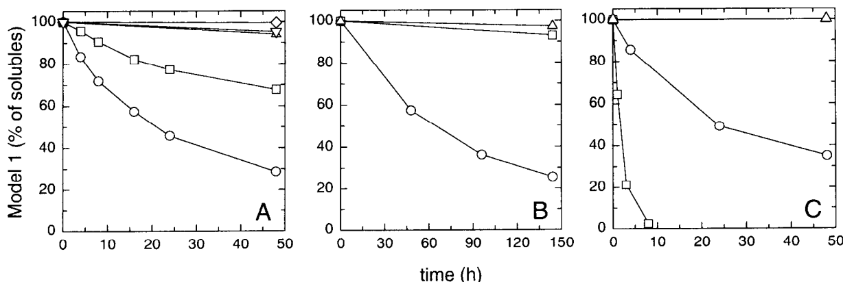
Fig. 1. Conversion of lignin model 1 to soluble products by peroxy radical-generating systems. Samples were analyzed by HPLC as described (Section 2.3), and the data are expressed as ( 14 C in model 1/total 14 C in the chromatogram) × 100. A: Reactions with MnP, Mn(II), and linoleic acid: complete reaction (○), reaction minus MnP (△), reaction minus Mn(II) (▽), reaction minus linoleic acid (◇), complete reaction plus catalase (●). B: Reactions with H 2 O 2 , Fe(II), and arachidonic acid: complete reaction (○), reaction minus H 2 O 2 and Fe(II) (●), reaction minus arachidonic acid (△). C: Reactions with azo compounds: reaction with ACVA (○), reaction with AMPD (●), reaction without azo compound (△).
