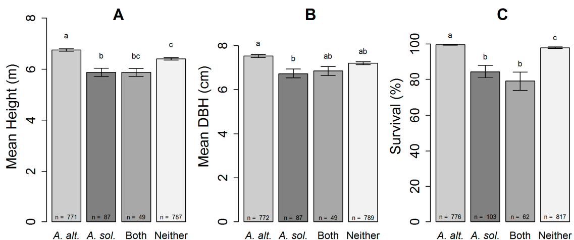
Figure 2. (A) The mean height, (B) mean diameter at breast height (DBH), and (C) percent survival among western white pine ( Pinus monticola ) growing in association with Armillaria altimontana ( A. alt. ), A. solidipes ( A. sol. ), both A. altimontana and A. solidipes (Both), or neither Armillaria species (Neither) at 16 years post-planting at the Priest River Experimental Forest, northern Idaho, USA. The height and DBH measures were not available for every live tree in the dataset. The bars show the standard error. Means sharing a lower case letter within each bar graph (i.e., A, B, and C) are not significantly different ( p < 0.05 ) by Tukey-adjusted means separation.
