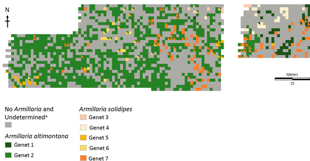
Figure 1. The Armillaria species and genet distribution within the Ida Creek plantation (0.8 ha) at the Priest River Experimental Forest, Idaho, USA: Each square pixel represents 1.2\text{ m} \times 1.2\text{ m} (a single tree location), and the colored pixels indicate trees associated with Armillaria altimontana , A. solidipes , or both. Cells split diagonally show the two unique genets that were identified on that single tree. The grey pixels indicate trees where neither A. altimontana nor A. solidipes were found or trees that were either missing or died early from unknown causes. The sequences ( tef1 ) from G1–G7 (MH879011–MH879017) are deposited in GenBank.
