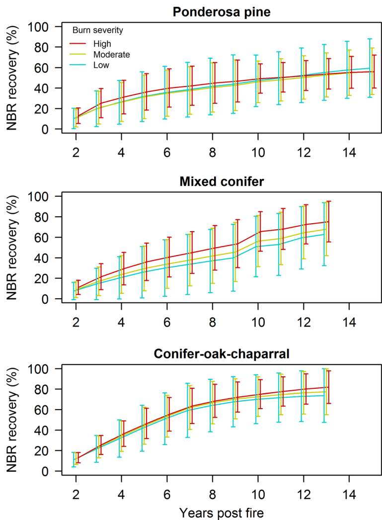
Fig. 4 Time series of percent recovery of mean percent Normalized Burn Ratio (NBR) for 12 wildfires in western North America that burned during the years 2000 to 2007. Bars show \pm 1 standard deviation. NBR recovery rates varied by severity, time since fire, and forest type
