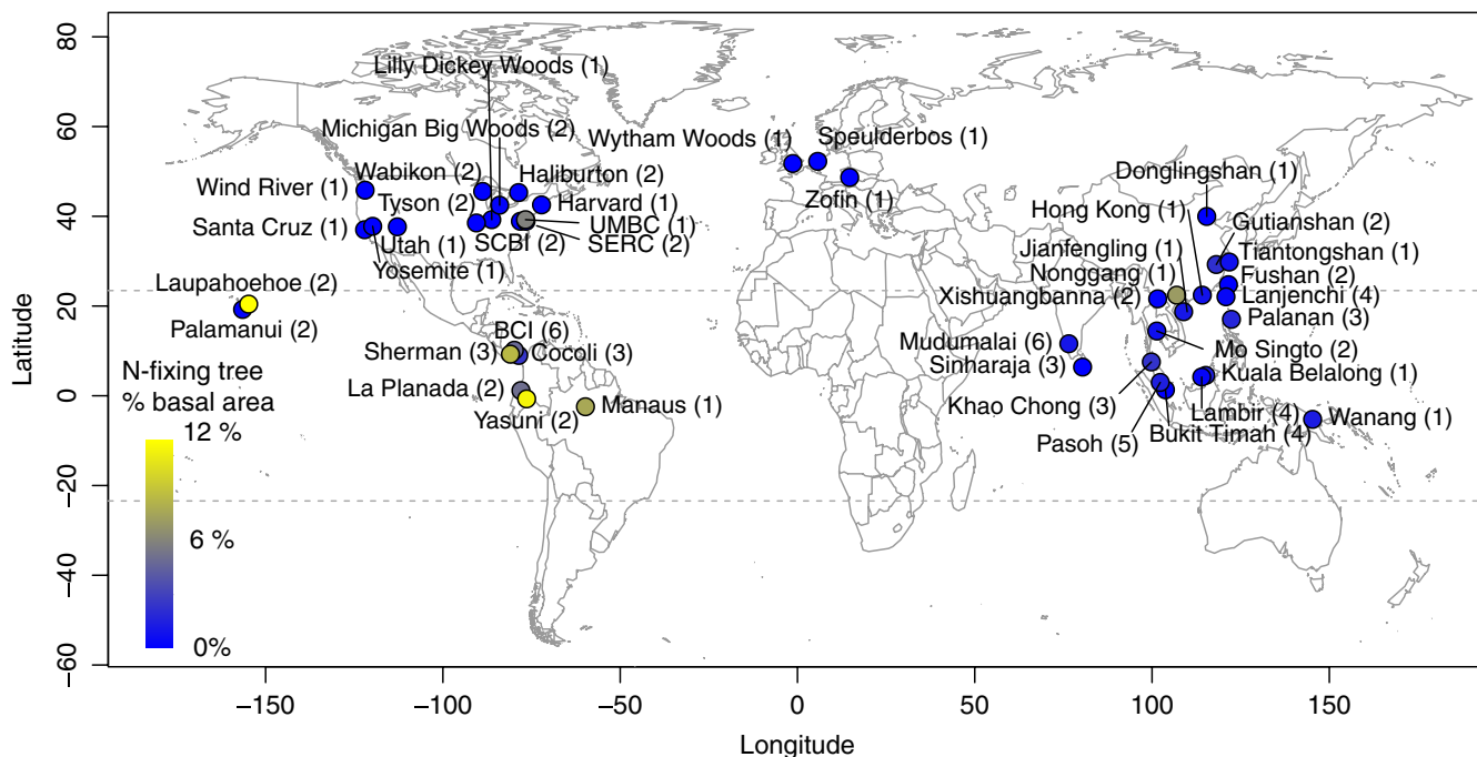
FIGURE 1 Map showing locations and N-fixing tree abundances of the 44 CTFS-ForestGEO plots. Each plot is represented by a circle, together with its name and the number of censuses (in parentheses). UMBC, SCBI, SERC and BCI stand for University of Maryland, Baltimore County; Smithsonian Conservation Biology Institute; Smithsonian Environmental Research Center; and Barro Colorado Island respectively. Plot colour indicates the % of total tree basal area from N-fixing trees (see color bar), except that Laupahoehoe (20.5%) is off the color scale and is assigned the color corresponding to the highest value on the scale. The three plots in Panama and two plots in Hawaii are offset slightly for visual clarity. Dashed grey lines indicate the Tropics of Cancer and Capricorn, which are the lines used to divide tropical and extratropical plots [Colour figure can be viewed at wileyonlinelibrary.com ]
