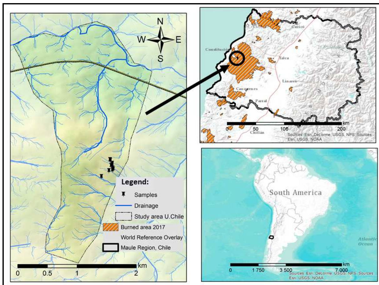
Fig. 1: Location of the study sites in the Justo Pastor León Research Station
