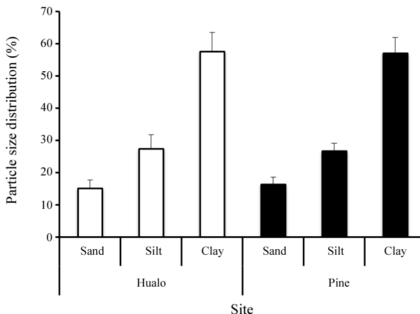
Fig. 2: Average and 90% confidence intervals of soil particle size distribution on both sites, in the first 10 cm depth
