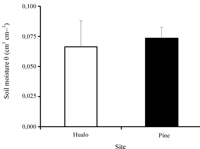
Fig. 3: Averages and 90% confidence intervals for volumetric soil water content ( \theta ), on both sites
