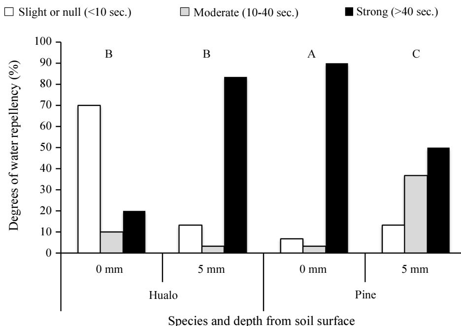
Fig. 4: Post-fire water repellency in the soil (%) relative to the depth of measurement and species, measured using the Water Drop Penetration Time (WDPT) method. Proportions within the graph followed by the same letter are not significantly different at the 0.10 level, evaluated using a Chi-square analysis
