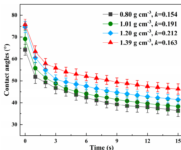
Figure 1. Contact angles of water as a function of time for scrimbers with various densities.
