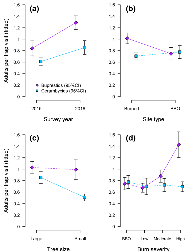
Fig. 4 Adult activity in relation to year (a), site disturbance type (b), tree size class (c), and burn severity (d), shown for two families of woodboring beetles on sites in the greater Sierra Nevada region of California, USA, sampled during the summers of 2015 and 2016. In (d), data from unburned, bark beetle outbreak (BBO) sites are compared with data from sites that burned at low, moderate, or high severity according to RdNBR classifications. Point estimates and error bars represent mean responses and 95% confidence intervals (CIs) from fits to models exemplified in Tables 9, 10, 11. Dashed lines connect means that do not differ significantly. Response variables are defined in Table 4 and predictor variables are defined in Table 5
