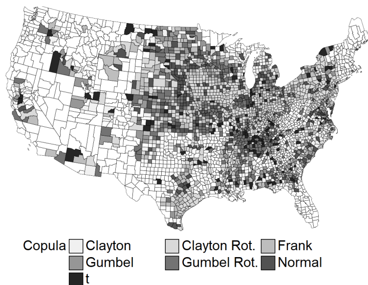
Figure 3. Best-Fitting Copula by County
