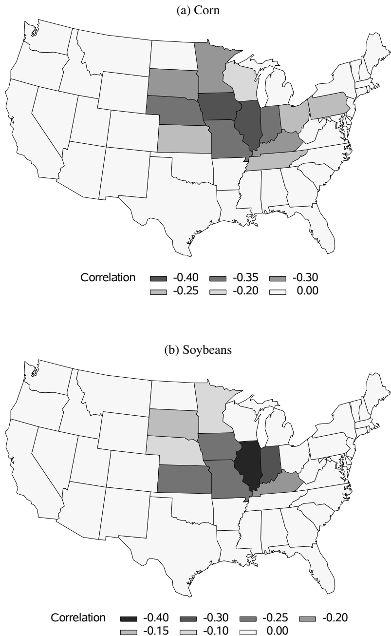
Figure 1. Pearson Correlation for Current Actuarial Methods
