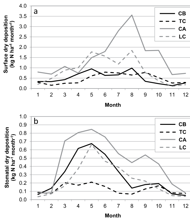
Fig. 1. Monthly mean (n = 2 years) of (a) surface and (b) stomatal deposition of atmospheric nitrogen estimated for the four Quercus ilex forests of the study.
