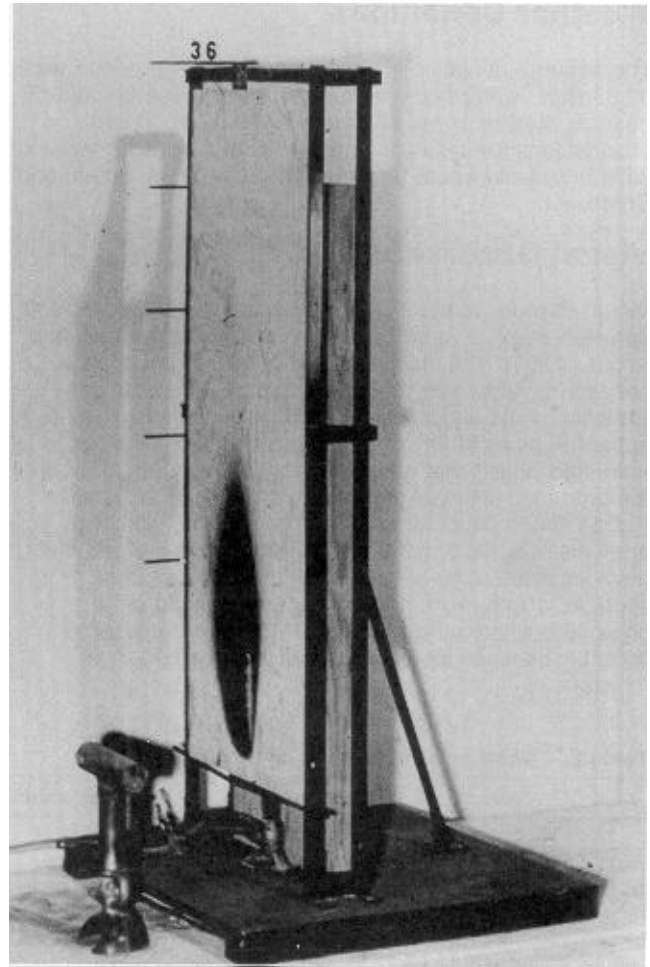
Figure 3.—Modified Schlyer test. (M85 0412)
