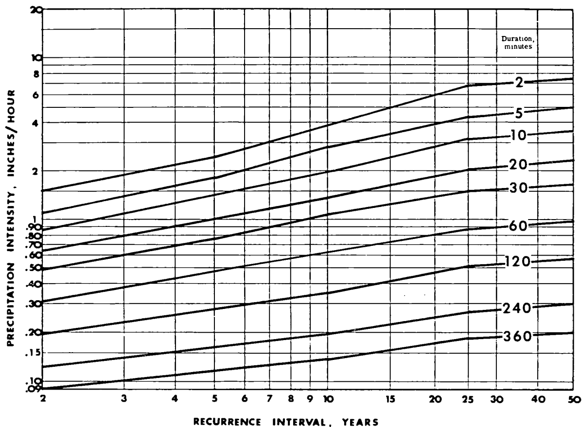
Figure 4.--Intensity-duration-frequency curves for recurrence intervals of 2 to 50 years and durations of 2 minutes to 6 hours for the Great Basin Experimental Area. Curves for precipitation Zone 1 are shown in 4a, Zone 2 in 4b, Zone 3 in 4c, and Zone 4 in 4d. (Log-extreme distribution)
