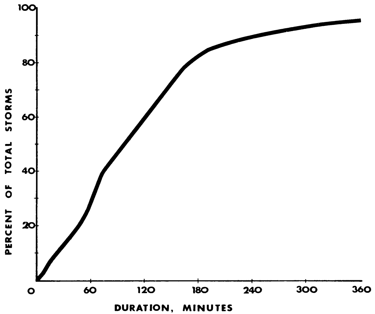
Figure 8.--Mass curve of accumulated percent of total storms by storm duration for precipitation Zone 4 of the Davis County Experimental Watershed.
