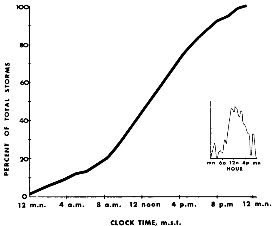
Figure 5.--Mass curve of accumulated percent of total storms by hour of storm beginning, for precipitation Zone 3 of the Great Basin Experimental Area. The inset is a schematic showing the distribution of storms by hour.
