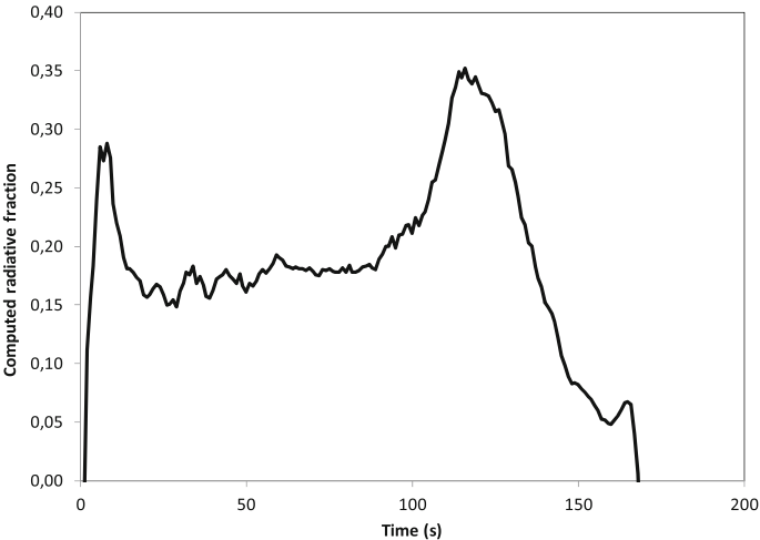
Figure 26. Computed radiative fraction for the case n3_20.
