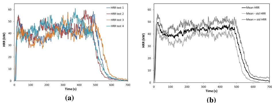
Figure 15. Results for the case 1_0 experiments. (a) Instantaneous HRR of the different replications (b) Mean HRR with the associated standard deviation.
