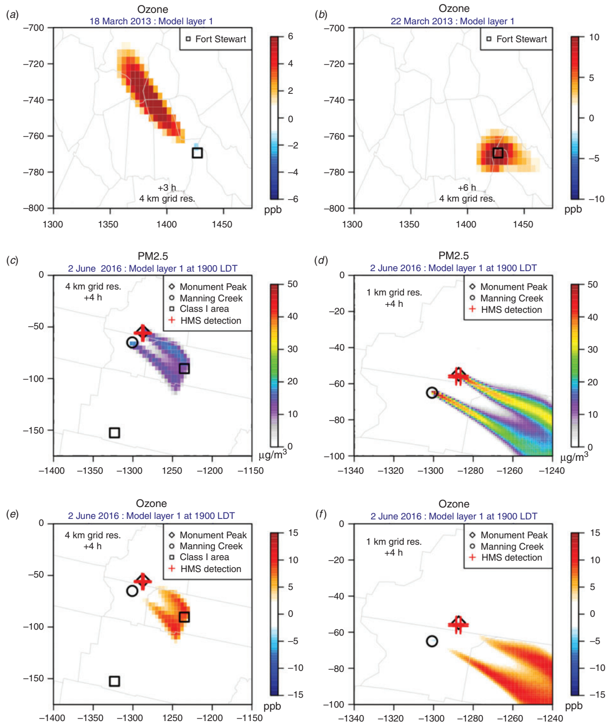
Fig. 10. CMAQ-BlueSky estimated O 3 (ppb) on (a) 18 March and (b) 22 March 2013 for a hypothetical 868 acre (approximately 350 ha) prescribed fire at Fort Stewart, GA. Model predicted PM 2.5 (c, d, µg m -3 ) and O 3 (e, f, ppb) are shown for an actual and planned burn unit at Fishlake NF, UT, on 2 June 2016, 4 h after ignition at both 4- and 1-km grid resolutions. NOAA Hazard Mapping System (HMS) satellite-based fire detections for the fire detections for the Monument Peak burn are also shown. LDT is local daylight time.
