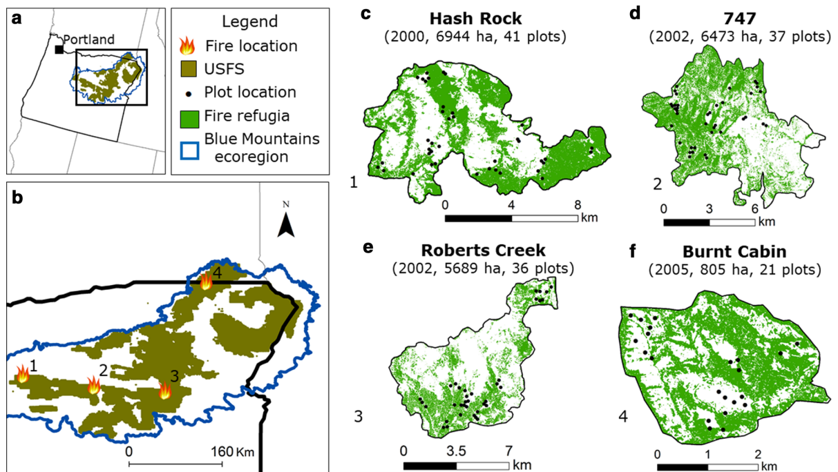
Fig. 1 The study area and study fires in central and northeastern Oregon. a The study was performed in the Blue Mountains ecoregion. b All four study fires burned primarily on land managed by the US Forest Service (USFS). c–f Fire refugia (green) within our four study fires, mapped using 1-m resolution aerial imagery, illustrate the complex spatial patterning of
