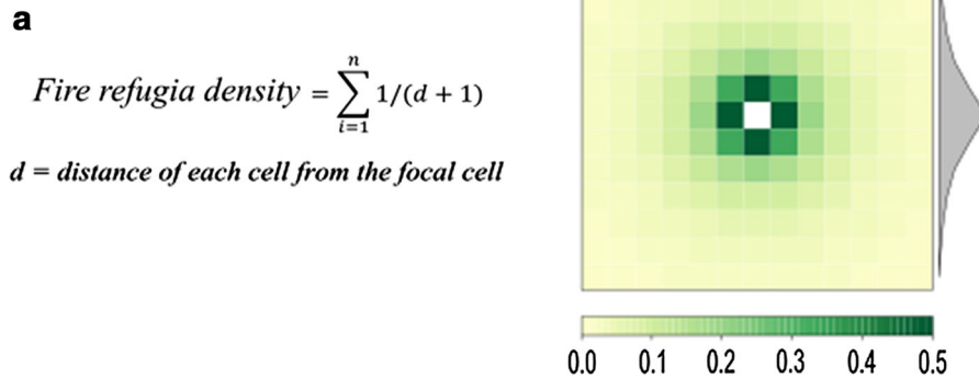
Fig. 2 a Fire refugia density was calculated by dividing the value of each cell (1 = refugia, 0 = non-refugia) by its distance from the focal cell and summing these values for the 300 \times 300 -m window. b Cell weights calculated with the refugia density approach for a reduced window size ( 6 \times 6 , plus an additional row-column pair for the focal cell). Distributions on the top and left demonstrate cell weights exponentially decreasing with
