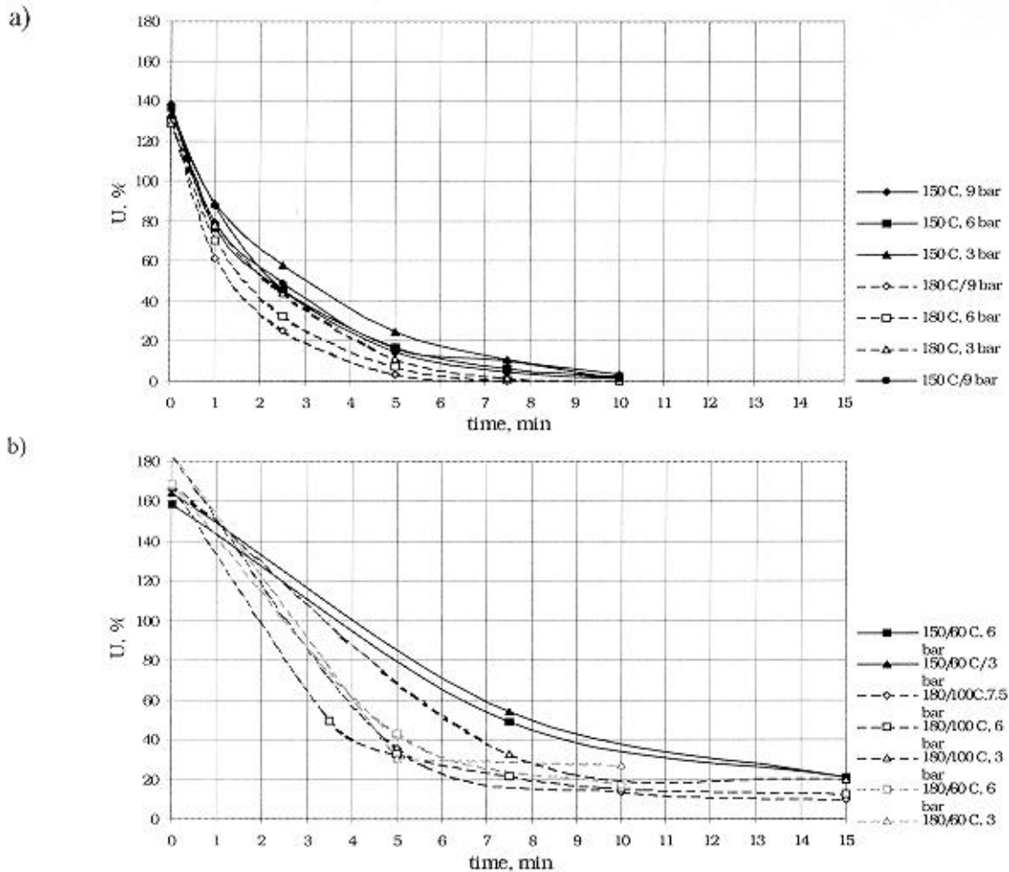
Figure 3. Drying curves for conventional drying (a) and condebelt drying (b)
