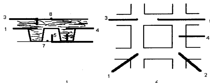
Figure 2. Location of thermocouples (Condebelt 1, 2, 3 and 5, conventional all)
