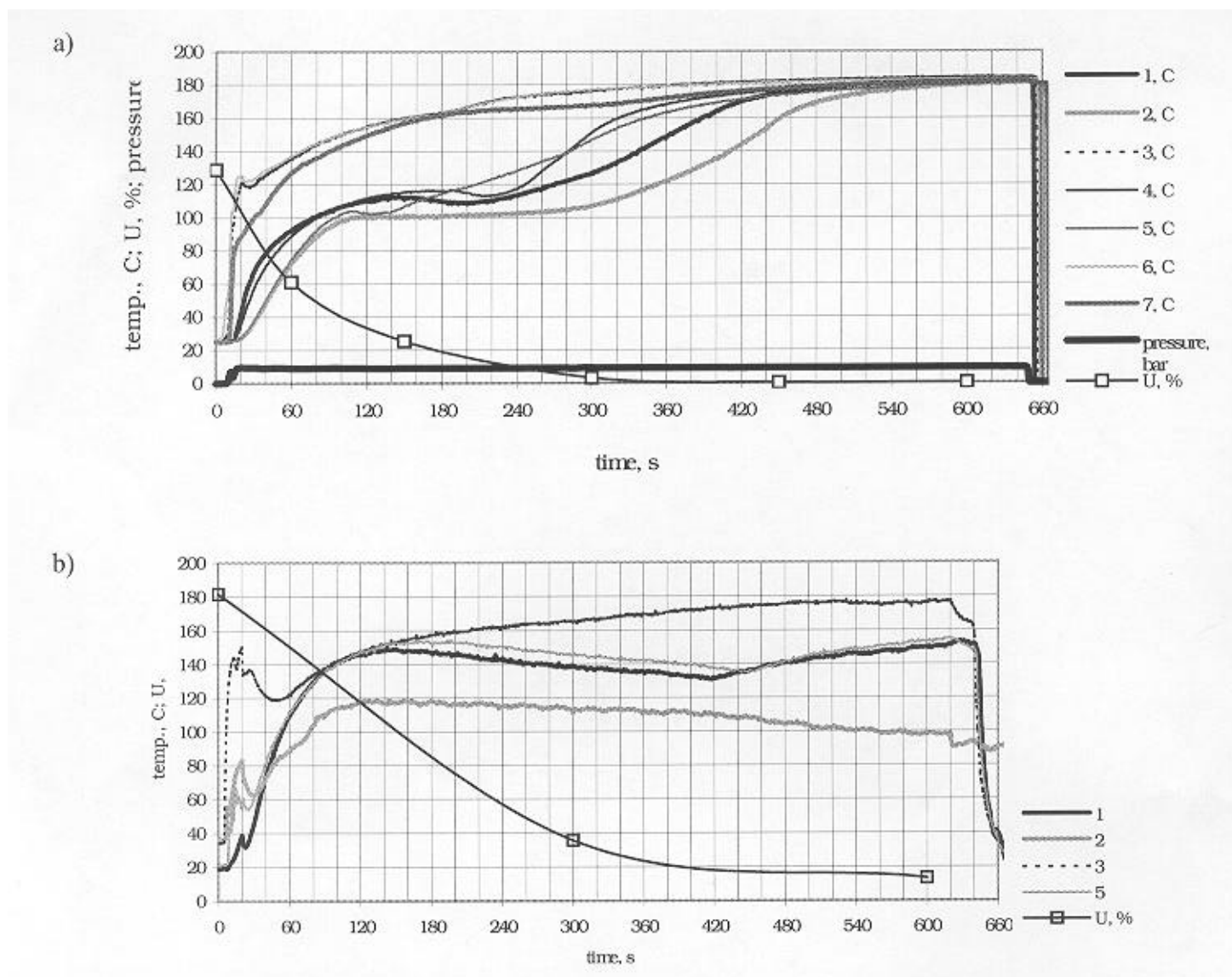
Figure 4. Temperature curves, a) conventional drying, b) Condebelt drying.
