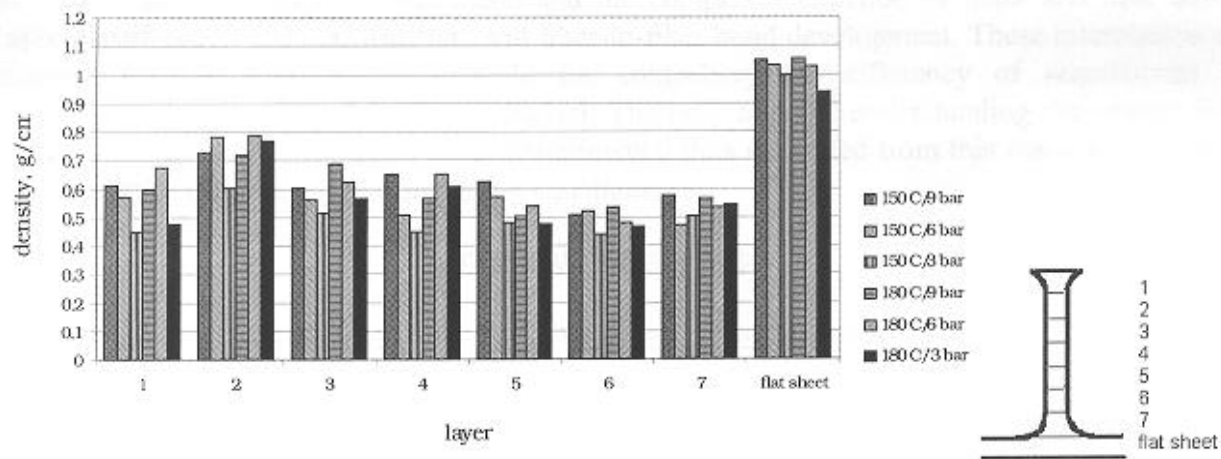
Figure 5. Conventional drying density distribution, 180 °C, 9 bar, 10 minutes.
