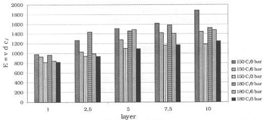
Figure 6. Sonic modulus of elasticity.
