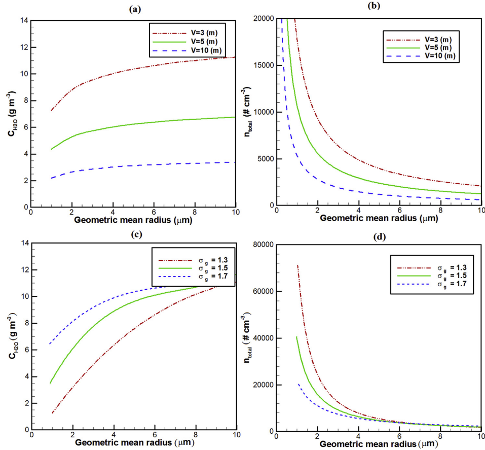
Fig. 5. Modelled relationships between liquid water content C_{H_2O} , geometric mean radius \bar{r}_g , geometric standard deviation \sigma_g and visibility V .
