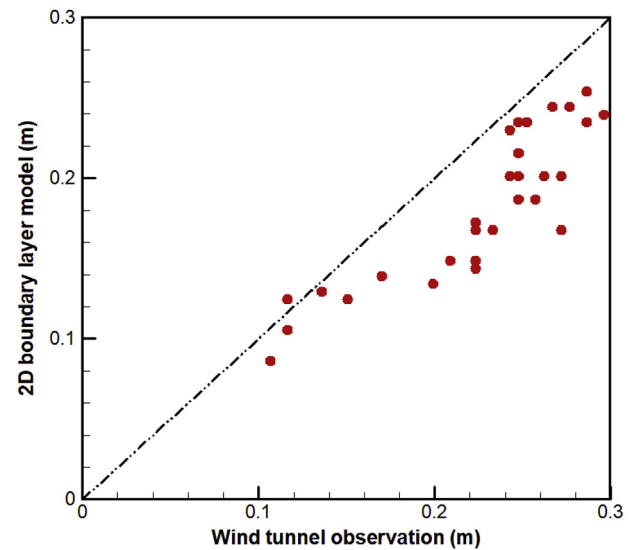
Fig. 8. Comparison of smog boundary layer height between 2D boundary layer model prediction and wind tunnel observation for the fog condition corresponding to liquid water content of 0.1 \text{ g kg}^{-1} .
