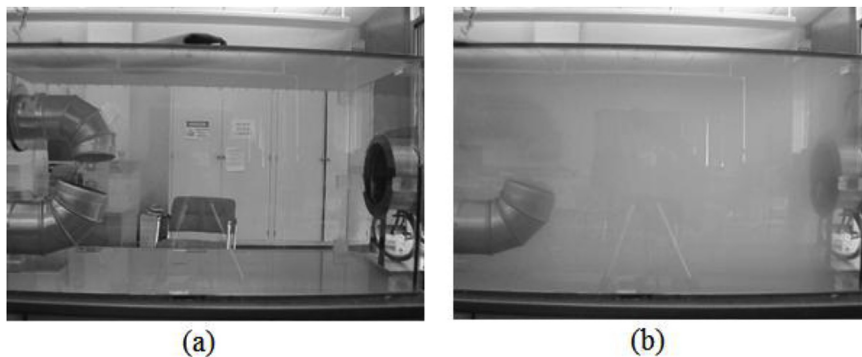
Fig. 6. Example of visibility reduction due to mixing of hot and cold moist air masses without presence of smoke.
