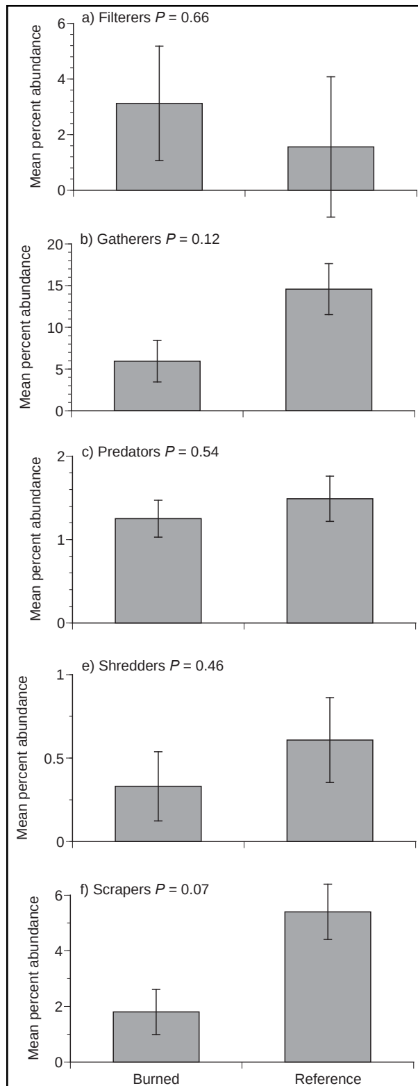
Figure 9. Mean percent abundance for functional feeding groups within burned and references streams in 2011. Error bars represent standard errors of the mean. \alpha = 0.05 .
