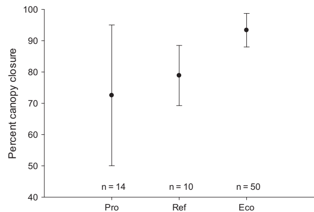
Fig. 3 Mean percent canopy closure and standard deviation for production forestry watersheds (Pro), reference watersheds (Ref), and ecological forestry watersheds (Eco)
