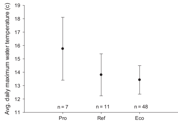
Fig. 2 Mean average daily maximum temperatures and standard deviation (9 July–16 August) for production forestry watersheds (Pro), reference watersheds (Ref), and ecological forestry watersheds (Eco)
