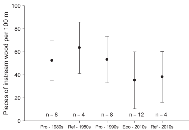
Fig. 4 Mean number of instream wood pieces per 100 (pieces 3 m and longer) and standard deviation for different times and types of management. Production forestry watersheds = Pro, reference watersheds = Ref, ecological forestry watersheds = Eco
