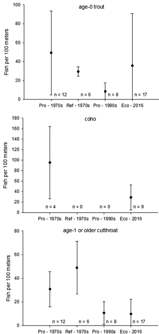
Fig. 5 Mean number of fish per 100 meters and standard deviation of three groups of fish (age-0 trout, coho, and age-1 or older cutthroat trout) for different time and management approaches. Production forestry watersheds = Pro, reference watersheds = Ref, ecological forestry watersheds = Eco
