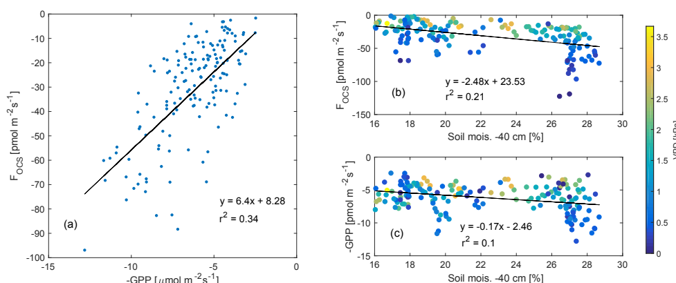
Figure 3. F_{\text{OCS}} was linearly correlated to GPP (plotted as a negative quantity to show ecosystem uptake a ), while both F_{\text{OCS}} and GPP reduced as a function of decreasing soil moisture ( b–c ). Data presented here are midday means; data in ( b–c ) are colored according to VPD.
