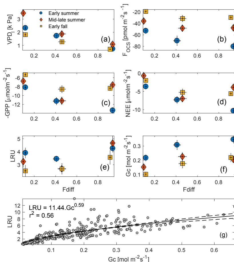
Figure 6. Midday VPD 1 , F OCS , NEE, and GPP plotted against the fraction of diffuse downwelling shortwave radiation (a–d) for early summer, mid–late summer, and early fall of 2015 (these periods are defined in Sect. 3.4). High values on the x axis indicate completely overcast or cloudy conditions, whereas as low values indicated clear skies. LRU increases with increasing f diff during each period, but the increase is most pronounced in the early summer (e). G c increases from clear to partly cloudy conditions across the three periods and plateaus during overcast sky conditions (f). Vertical bars indicate 1 SE. Across the three periods, LRU increased with G c and leveled off at G c values greater than \sim 0.5 \text{ mol m}^{-2} \text{ s}^{-1} (g).
