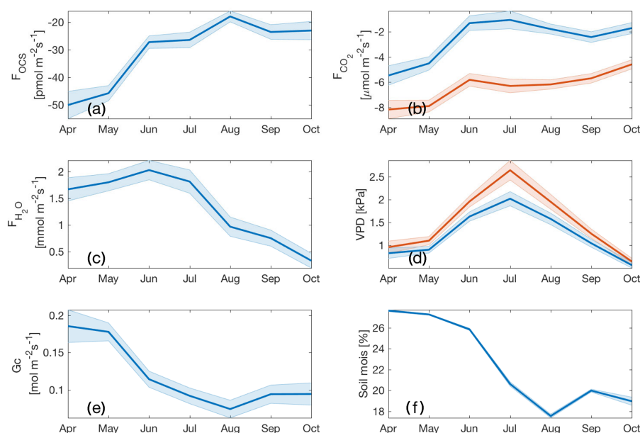
Figure 4. Monthly means for daytime F_{\text{OCS}} ( a ); NEE and GPP (blue and red curves; b ); water vapor flux ( c ); \text{VPD}_a and \text{VPD}_l (blue and red curves, respectively; d ); canopy conductance ( G_c ; e ); and soil moisture at -40 cm depth ( f ). Shaded regions indicate standard error.
