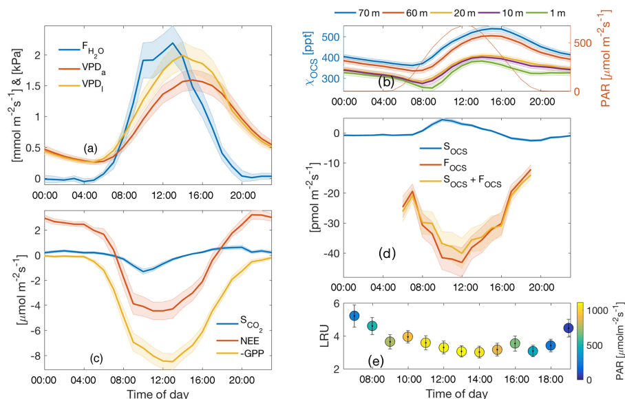
Figure 2. Diurnal cycle of measured H_2O flux (blue curve) and VPD estimated from air and leaf temperatures (red and yellow curves, respectively) (a); diurnal cycles of OCS mixing ratio profiles measured along the canopy (left axis) and mean PAR (right axis) (b); inferred storage flux of CO_2 (blue curve), measured turbulent flux of CO_2 (NEE; red curve), and estimated flux of GPP (yellow curve, plotted as a negative quantity to show uptake) are shown in (c); the diurnal cycle of change in storage flux of OCS ( S_{OCS} ; blue curve), the estimated flux of OCS using flux-gradient similarity ( F_{OCS-FG} ; red curve), and the sum of the two fluxes ( F_{OCS} ; yellow curve) (d); the mean diurnal cycle of leaf relative uptake estimated according to Eq. (4) (e) colored according to mean PAR. Shaded regions in (a–d) and vertical bars in (e) represent 1 standard error.
