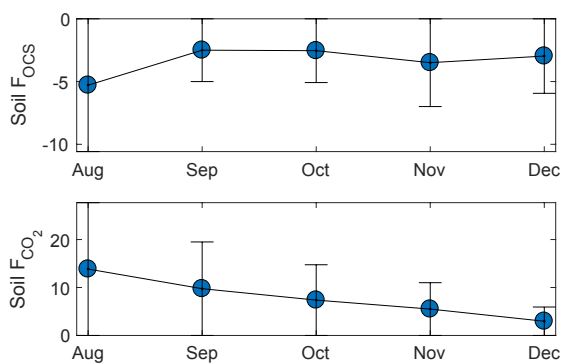
Figure 5. Surface F_{OCS} and F_{CO_2} from chamber measurements from sites 2 and 3. Site 1 was atypical (see Sect. 2.7), and therefore fluxes are not shown. Values for site 1 F_{OCS} and F_{CO_2} were -22 \pm 0.3 \text{ pmol m}^{-2} \text{ s}^{-1} and -83 \pm 2 \mu\text{mol m}^{-2} \text{ s}^{-1} , respectively. Error bars indicate standard deviation.
