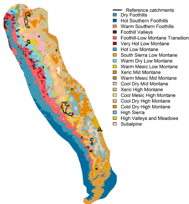
Fig. 5. Map of climate classes. Catchments containing at least one reference area indicated to illustrate the environmental distribution of reference areas.
