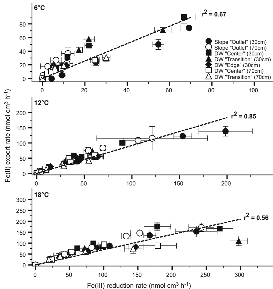
Fig. 3 Correlation between steady-state potential Fe(III) reduction rates and Fe(II) export rates (nmol cm 3 h -1 ) for the slope and depressional wetlands measured at 6, 12 and 18 °C. The dashed lines are the linear regressions ( r^2 ) representing the
