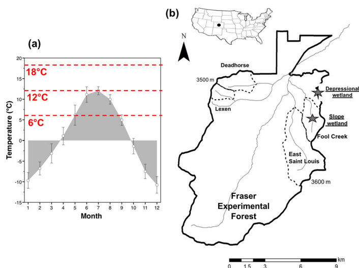
Fig. 1 a Average monthly air temperature from 1976 to 2003 at the USFS Fraser Experimental Forest derived from hourly temperature measurements (Elder 2006). Error bars show standard deviations over the period 1976–2003. Red dashed lines denote the temperatures used for the flow-through experiments (FTR). b Wetland locations at the USFS Fraser Experimental Forest in the Rocky Mountains, Colorado, USA.
