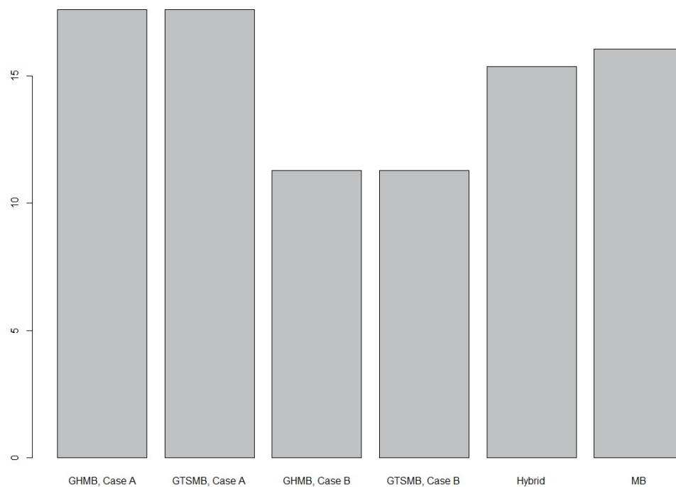
Figure 4. The average relative standard error for the different methods, [%].
