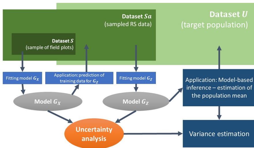
Figure 1. Overview of Generalized Hierarchical Model-Based estimation.
