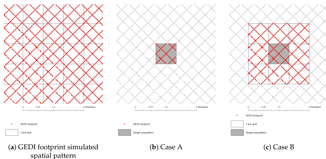
Figure 3. (a) Simulated spatial pattern of GEDI footprints and the 1-km grid delineation; (b) Case A: data for a single 1-km grid-cell were used; (c) Case B: data from neighboring grid-cells were used as well, for the GHMB and GTSMB estimators.
