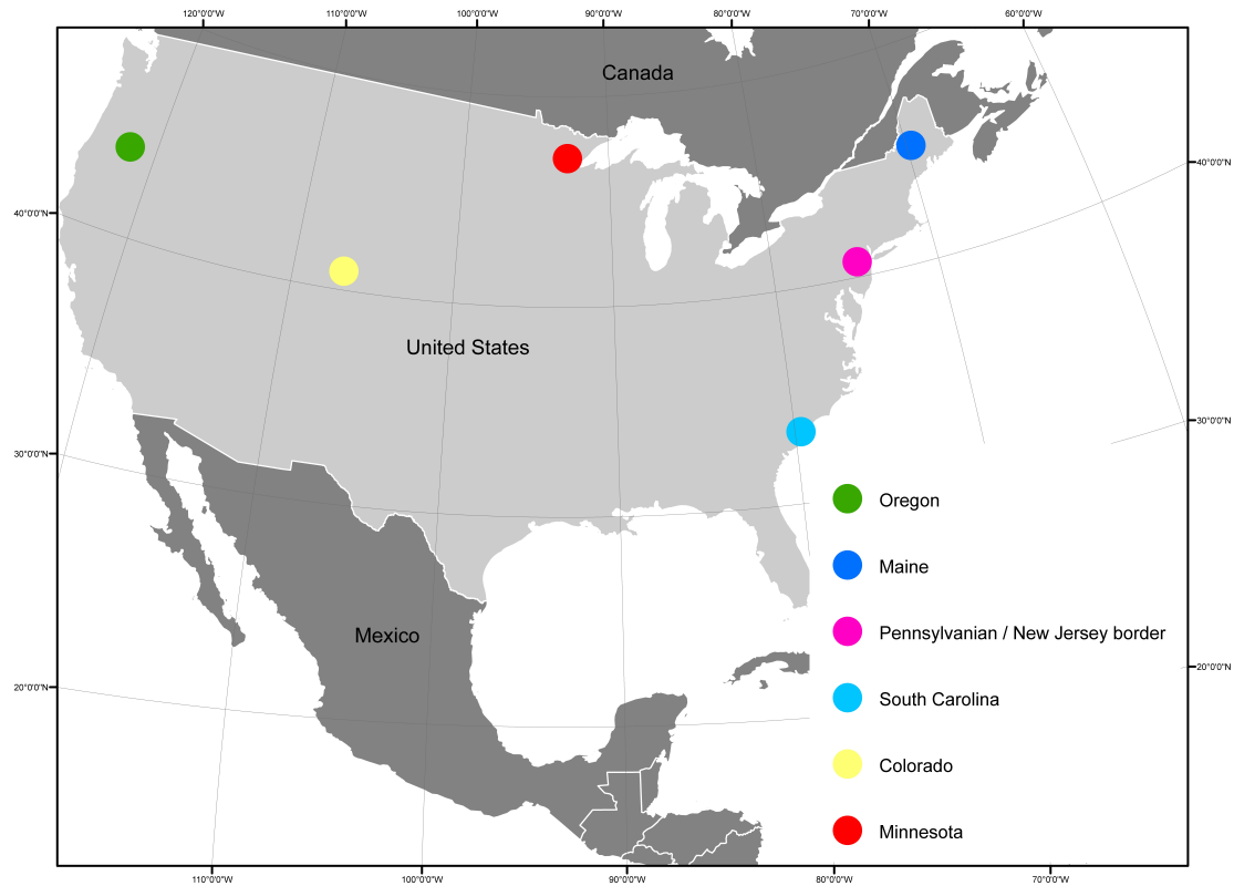
Figure 2. Study sites across the USA.
