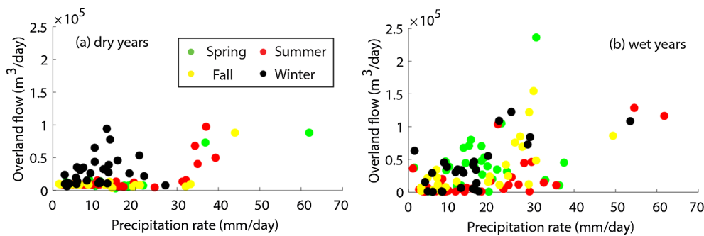
Fig. 6. Daily overland flow (unit: \text{m}^3/\text{day} ) associated with different precipitation intensities (unit: \text{mm}/\text{day} ) during (a) dry years and (b) wet years. Dots of different color indicate seasonal overland flow rates. (For interpretation of the references to color in this figure legend, the reader is referred to the web version of this article.)
