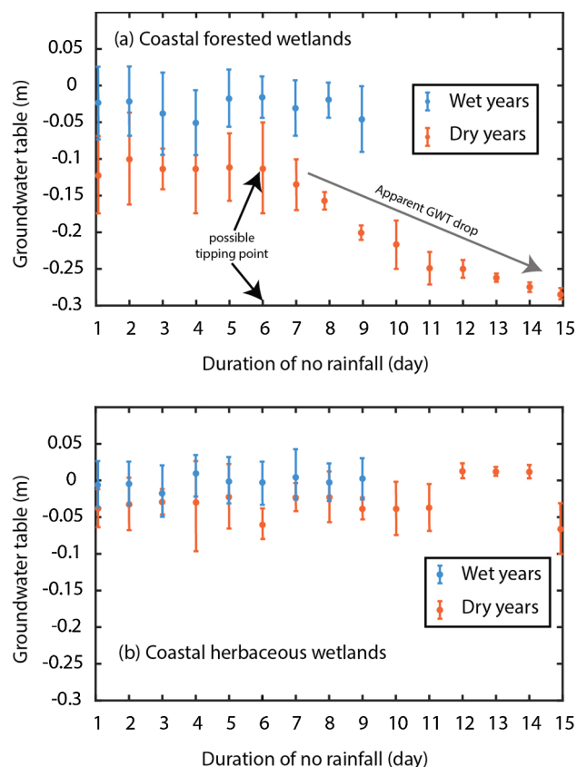
Fig. 5. The mean GWT (m) under the different duration of no rainfall for (a) coastal-forested wetland and (b) coastal herbaceous wetland, respectively. Each bar represents the averaged GWT under drought events with the same duration. The dots in the middle of the bars indicate the mean GWT, and the ends of the bars represent one standard deviation from the mean GWT.
