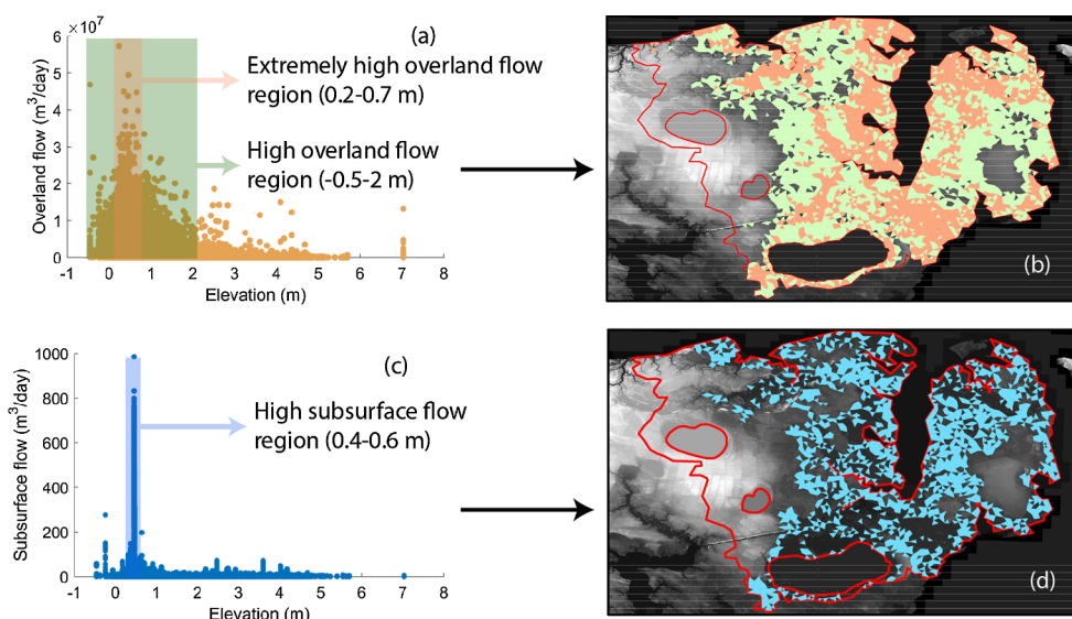
Fig. 7. Distribution of overland and subsurface flow rates (unit: \text{m}^3/\text{day} ) during large rainfall events (higher than the 75th percentile of the 30 years' rainfall distribution) from 1995 to 2014. (a) Overland flow rate on each model cell at different elevations. Each dot represents each model cell. Green and orange shaded zones indicate the cells with high and extremely high overland flows, respectively. (b) Geographic distribution of the cells with high and extremely high overland flows. The green and orange cells are corresponding to the cells in the green and orange zones in (a). The gray background is the elevation map with higher elevation in white and low elevation in black. The red line denotes the model boundary. (c) is the same as (a) but for subsurface flow. The light blue shaded zone highlights the cells with the high subsurface flow. (d) is the same as (b) but for subsurface flow. The light blue cells are corresponding to the cells in the light blue zone in (c). (For interpretation of the references to color in this figure legend, the reader is referred to the web version of this article.)
