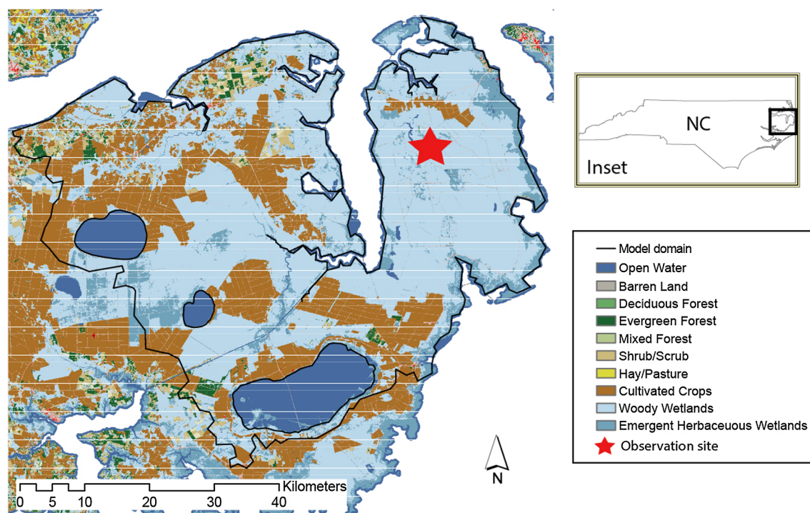
Fig. 2. The study area (35°24'48"N, 76°40'15"W - 36°5'11"N, 75°40'33"W) with land cover types. The red star indicates the observation site (35°46'34"N, 75°54'12"W). Inset: the location of the study area in North Carolina (NC). The black box in the inset indicates the study area. (For interpretation of the references to color in this figure legend, the reader is referred to the web version of this article.)
