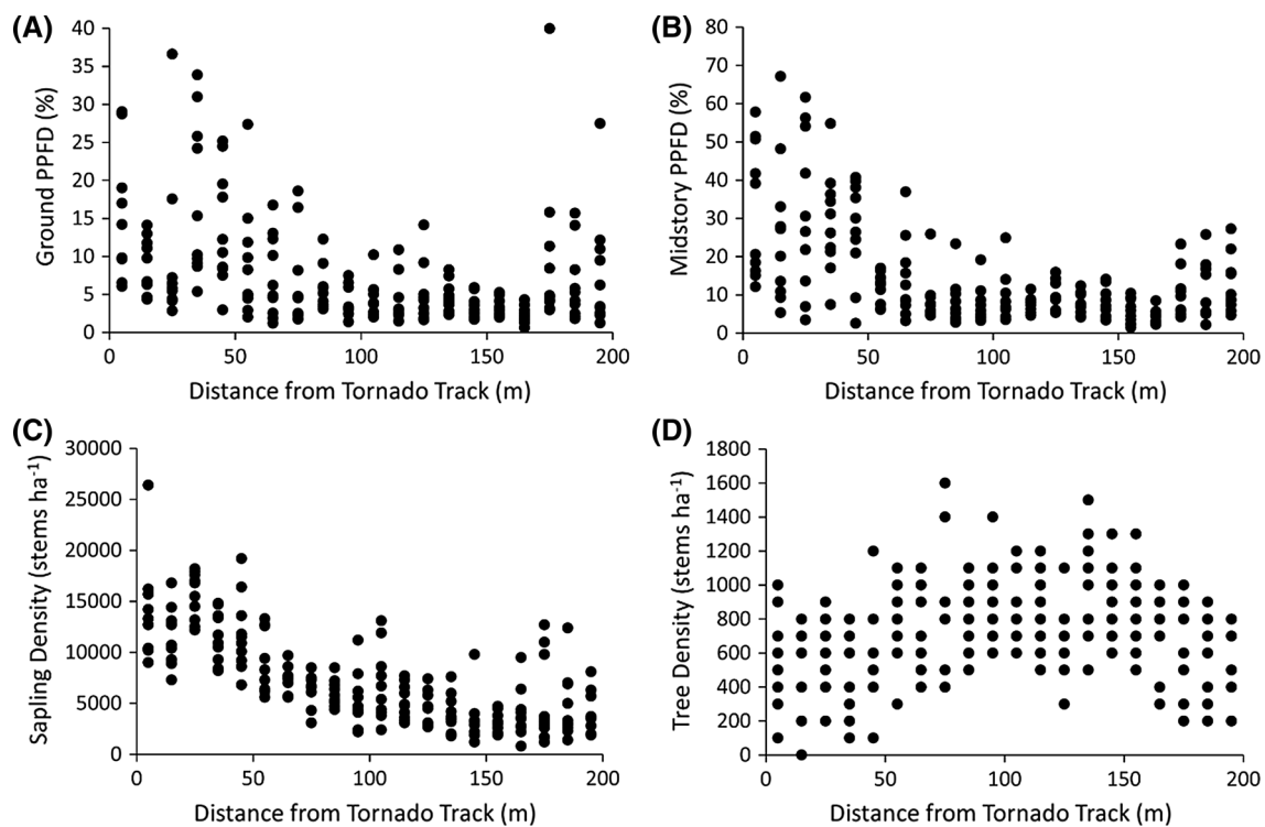
Fig. 2 Representations of changes in vertical light and stand structure with decreased distance from the tornado track. Ground PPFD (a) and midstory PPFD (b) tended to increase with increased disturbance and had greater heterogeneity in light intensity compared
