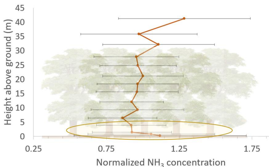
Figure 4. In-canopy vertical profiles of \text{NH}_3 concentration in two mixed hardwood forests in North Carolina. Height-wise \text{NH}_3 measurements for individual profiles have been normalized by the corresponding profile mean and then averaged for all profiles. Error bars represent \pm 1 standard deviation. Averages represent daytime profiles only. Coweeta results comprise n = 19 daytime profiles collected during summer 2016. Duke Forest results comprise n = 23 daytime profiles measured during summer 2009. Individual profiles were measured over 3 – 4 hour periods using phosphorous acid coated annular denuders. Circled regions show decreasing concentration just above forest floor indicative of emission.
