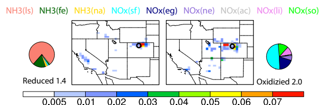
Figure 7. Same as Fig. 5 but for oxidized and reduced nitrogen deposition in RM. Units for the pie charts and colorbar are \text{kg N ha}^{-1} \text{ yr}^{-1} . The sum of the oxidized and reduced Nr deposition is smaller than the inset number in Fig. 5 because the number here excludes Nr from “other species”.
