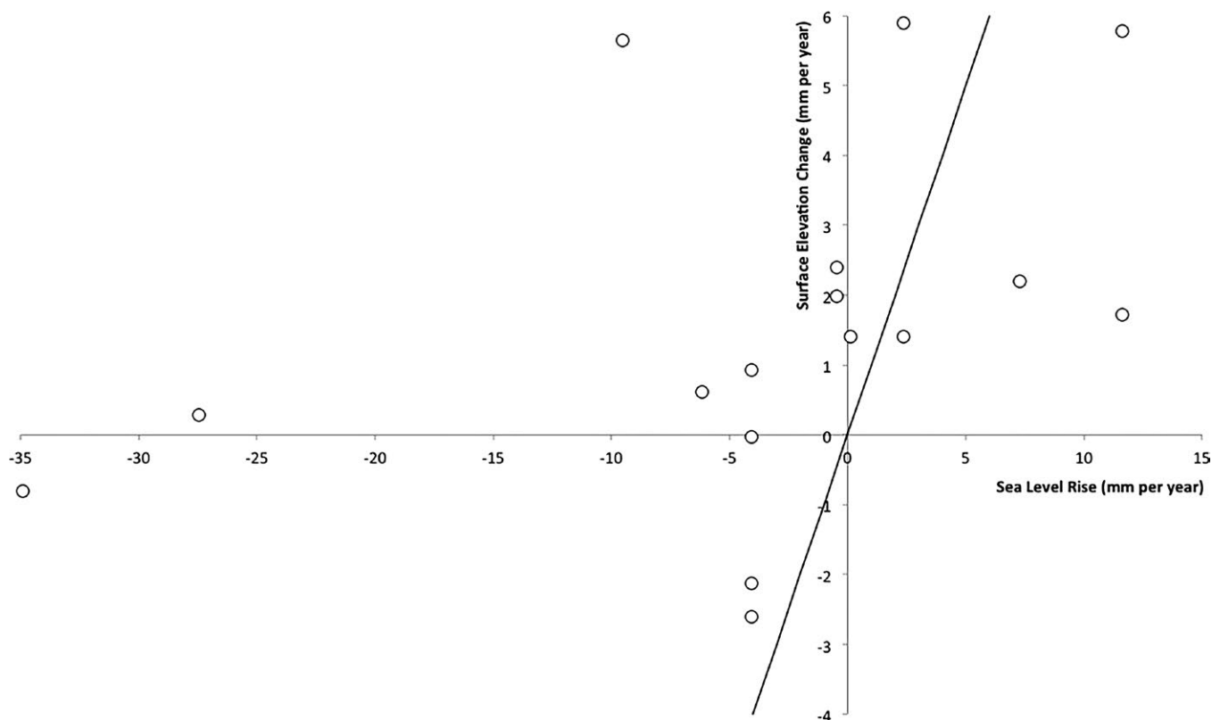
Fig. 5. A comparison of surface elevation change rates and SLR (recorded over the same time period) for various sites in East and South Australia. Black line = 1:1 line. Sites to the left of the line show a rate of elevation change greater than local SLR. Sites to the right of the line show a rate of elevation change lower than local SLR. Sources: Lovelock et al. (2011, 2015a,b), Rogers et al. (2006, 2013, 2014b).
