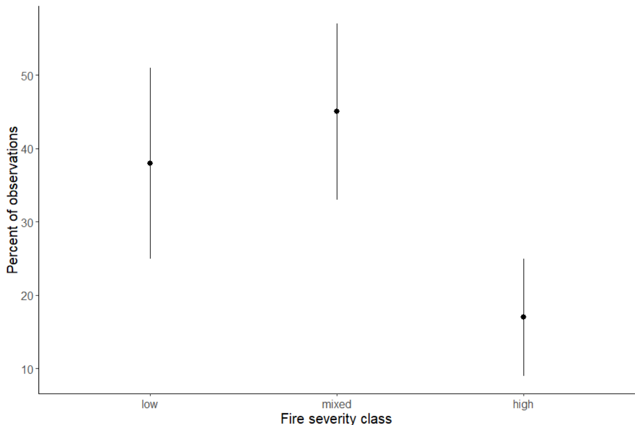
Figure 8—Mean percentage of observations (circles with \pm standard error bars) of fire severity class from seven fire history studies on ponderosa pine sites in Colorado.
