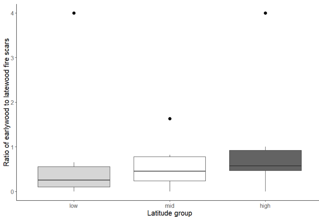
Figure 11—Variability in the ratio of earlywood to latewood fire scars by three latitude groups ( n = 12 for each group) from seven fire history studies in Colorado ponderosa pine ecosystems. See figure 7 for explanation of symbols.
