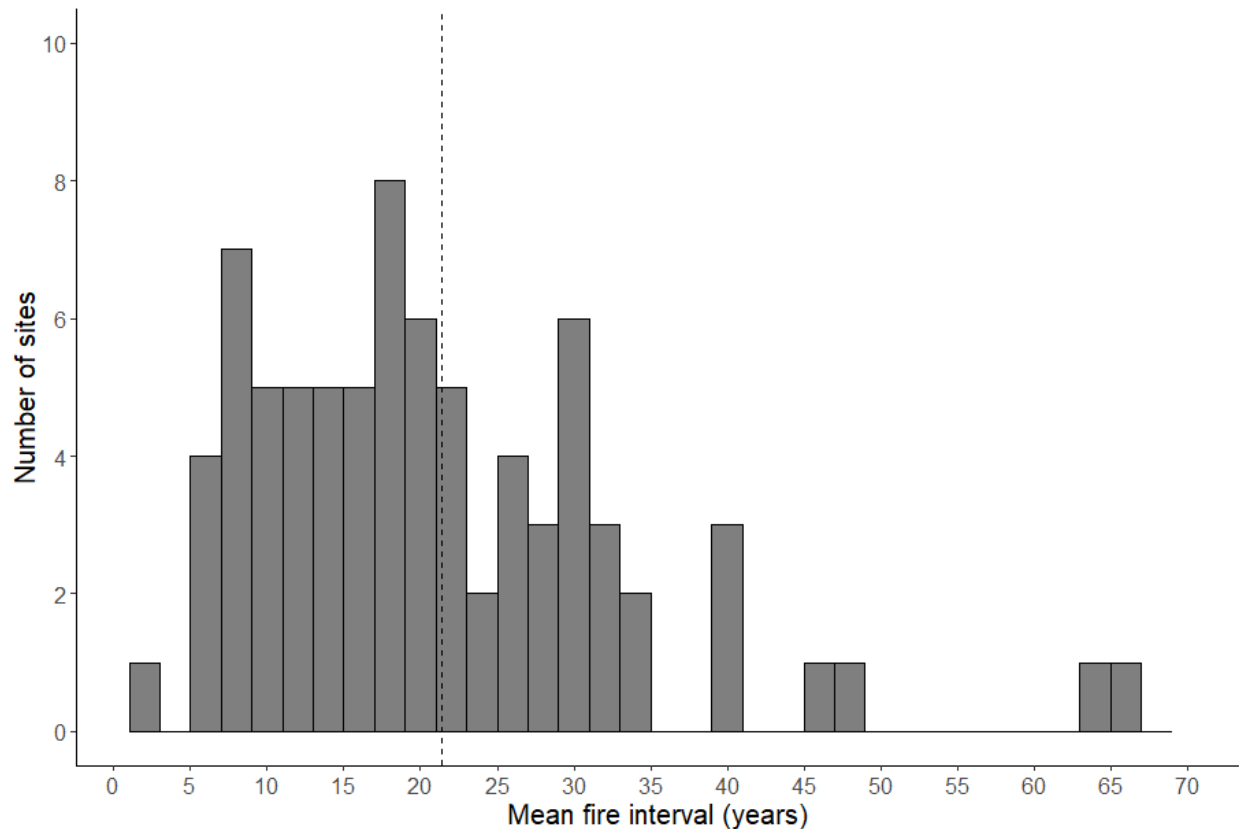
Figure 3—Frequency distribution of site-level MFI ( n = 78 ) from 17 studies in Colorado ponderosa pine ecosystems used in the meta-analysis. Vertical dashed line indicates overall mean.
