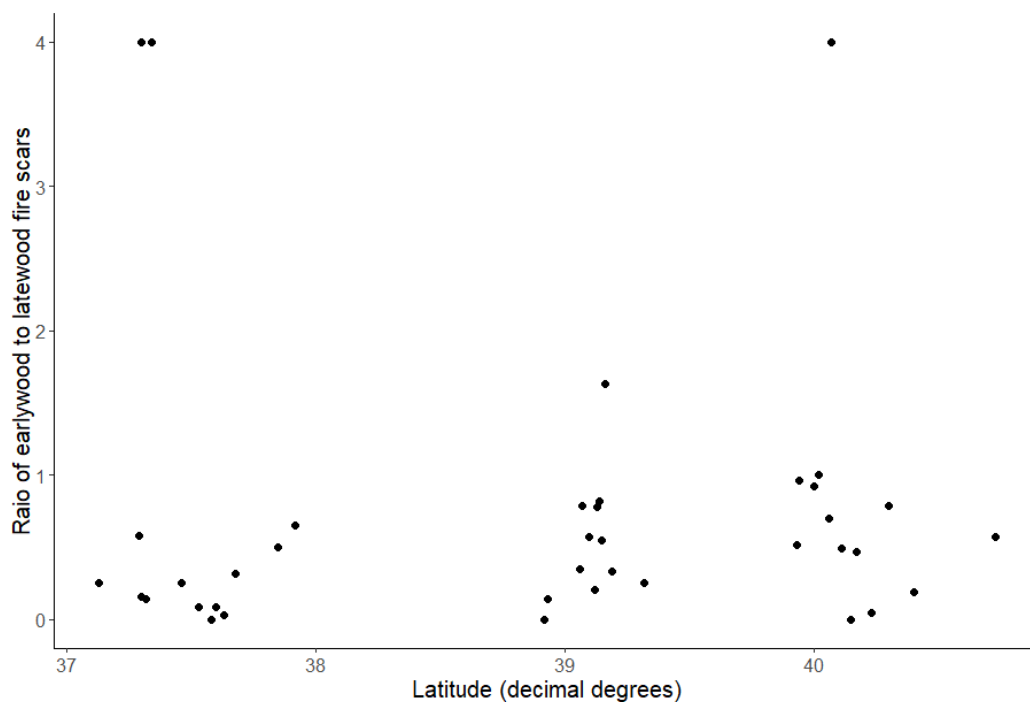
Figure 10—Relationship between the ratio of the percentage of earlywood fire scars to latewood fire scars and site latitude (decimal degrees) from seven fire history studies in Colorado ponderosa pine ecosystems ( n = 39 sites).
