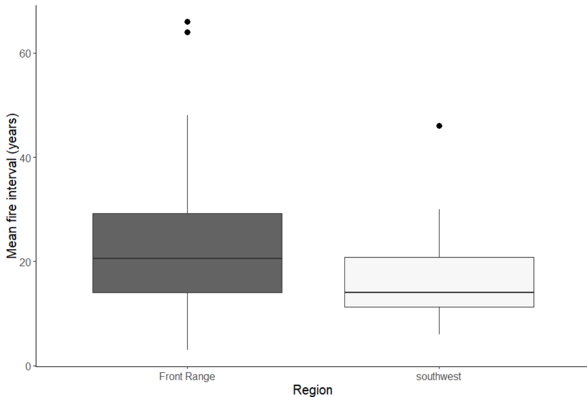
Figure 7—Variability of site-level mean fire-return intervals by two geographic regions (Front Range, n = 56 ; and southwestern, n = 22 ) from 17 fire history studies on ponderosa pine sites in Colorado. The line in the middle of each box represents the median value (50 th percentile), the ends of the boxes are the first (Q1) and third (Q3) quartiles, which cover the central 50% of the data, and the difference between Q3 and Q1 is the interquartile range (IQR). Vertical lines extend to the most extreme data points that are no more than \pm 1.5 \times \text{IQR} , and outliers beyond the lines are individually displayed as circles.
