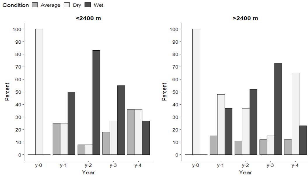
Figure 14—Relationship between fire year and antecedent precipitation conditions for two elevation groups (< 2,400 m, n = 12 and > 2,400 m, n = 27 ) from 12 fire history studies in Colorado ponderosa pine ecosystems. See figure 13 for axes descriptions.
