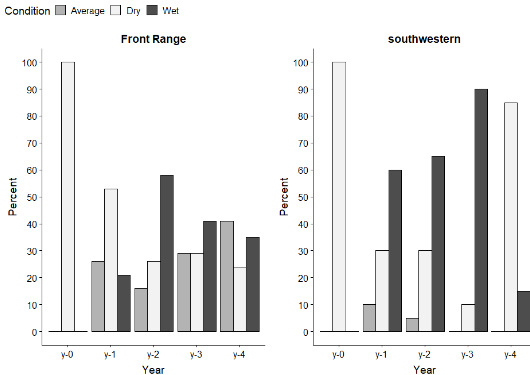
Figure 15—Relationship between fire year and antecedent precipitation conditions for two geographic regions in Colorado (Front Range, n = 19 and southwestern, n = 20 ) from 12 fire history studies in ponderosa pine ecosystems. See figure 13 for axes descriptions.
