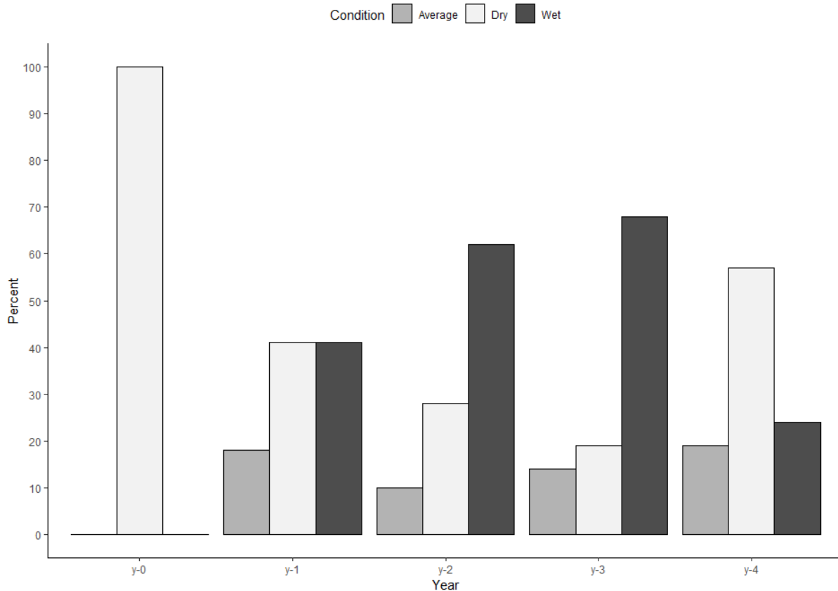
Figure 13—Relationship between fire year and antecedent precipitation conditions from 12 fire history studies in Colorado ponderosa pine ecosystems. Y-axis is the percent of all observations in each of three precipitation conditions: average precipitation, dry (below average), and wet (above average). Precipitation condition is derived from a combination of climate indices including Palmer Drought Severity, tree ring growth, NINO3 sea surface temperature, and others. X-axis is the year relative to fire year (y-0 is fire year, y-1 is year before fire year, etc.).
