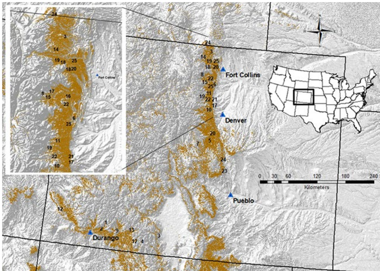
Figure 2—Distribution of ponderosa pine ecosystems in Colorado based on LANDFIRE Biophysical Settings [30]. Numbers indicate approximate location of studies used in this meta-analysis and correspond to references presented in table 1. For studies with more than one research site in close proximity, the approximate midpoint is shown. For studies with more than one site that spanned broad distances, the two distant endpoints are indicated with the same number. The map inset depicts a close up of the northern area where some sites were too close to display separately on the larger map.
