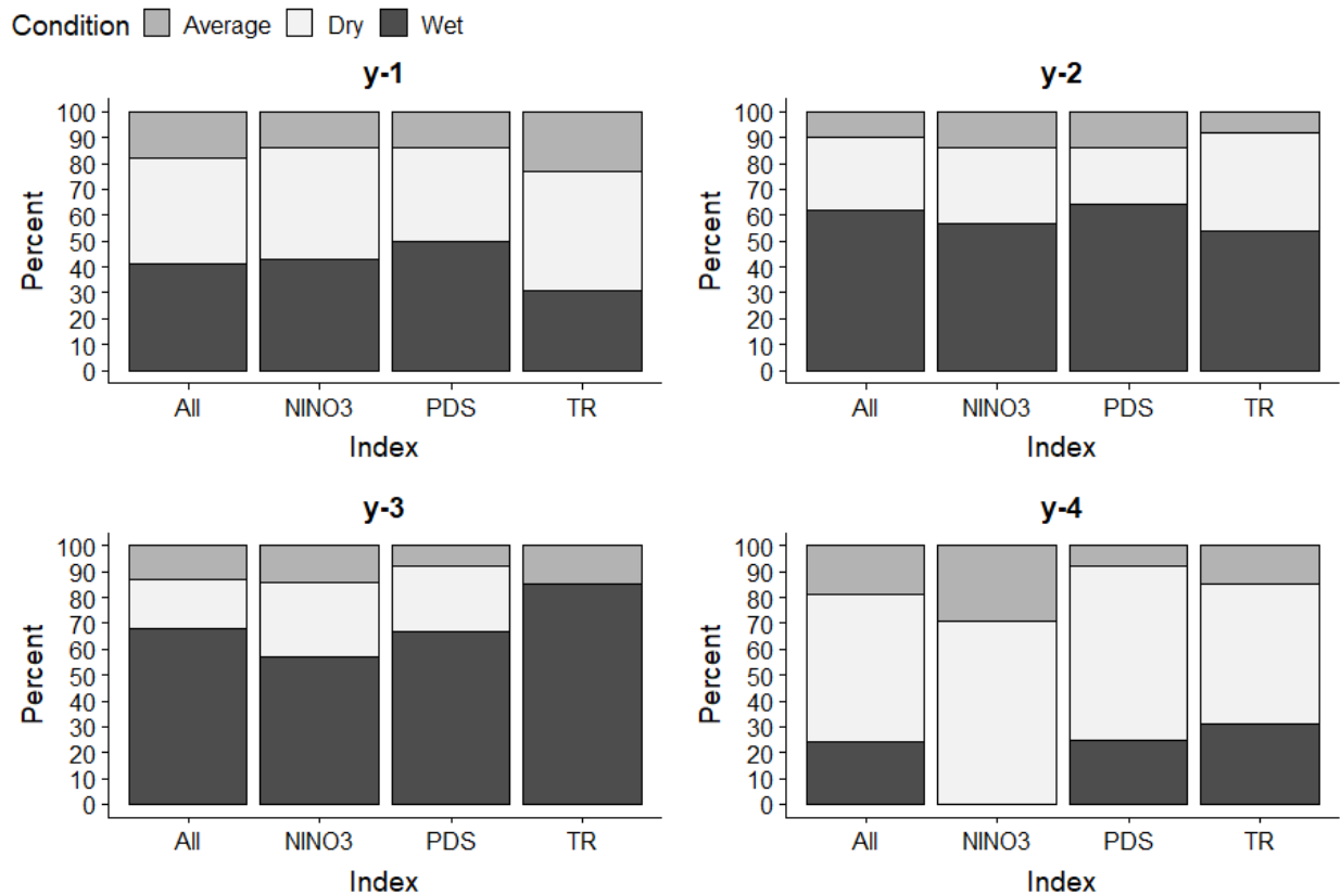
Figure 12—Comparison of three climate indices used to evaluate the relationship between fire year and antecedent precipitation conditions from 12 fire history studies in Colorado ponderosa pine ecosystems. Y-axis is the percent of all observations in each of three precipitation conditions: average, dry (below average), and wet (above average). Index categories are All, the combination of precipitation indices ( n = 39 ); NINO3, sea surface temperature index ( n = 7 ); PDS, Palmer Drought Severity index ( n = 14 ); and TR, tree ring growth index ( n = 13 ). The four panels represent the number of years preceding a fire year (y-1, one year prior; y-2, two years prior, etc.).
