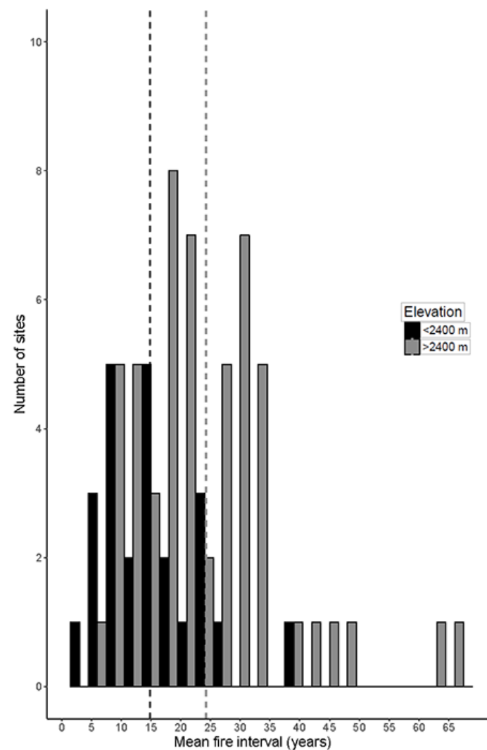
Figure 5—Frequency distribution of site-level mean fire intervals (MFI) from study sites below ( n = 24 ) and above ( n = 54 ) 2,400 m elevation. Vertical dashed lines indicate corresponding elevation group means.
