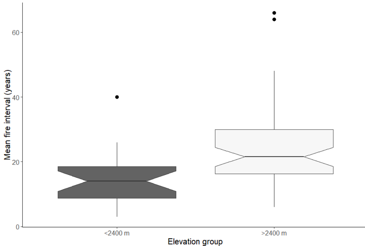
Figure 6—Variability of site-level mean fire intervals by two elevation groups (< 2400 m, n = 24 ; and >2400 m, n = 54 ) from 17 fire history studies on ponderosa pine sites in Colorado. The horizontal line in the middle of each box represents the median value (50 th percentile), the ends of the boxes are the first (Q1) and third (Q3) quartiles, which cover the central 50% of the data, and the difference between Q3 and Q1 is the interquartile range (IQR). The notches are an approximation of the 95% confidence interval for the median values. Vertical lines extend to the most extreme data points that are no more than \pm 1.5 \times \text{IQR} , and outliers beyond the lines are individually displayed as circles.
