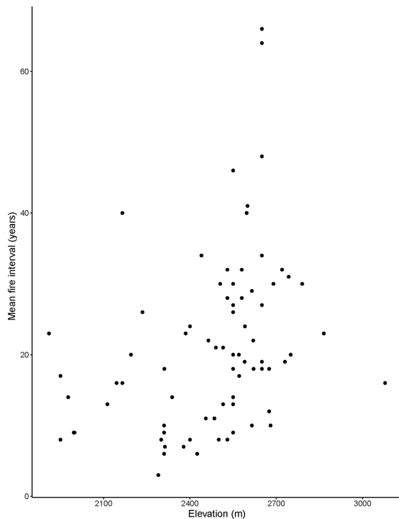
Figure 4—Relationship between site-level mean fire interval (MFI) and elevation for 78 ponderosa pine sites in Colorado.
