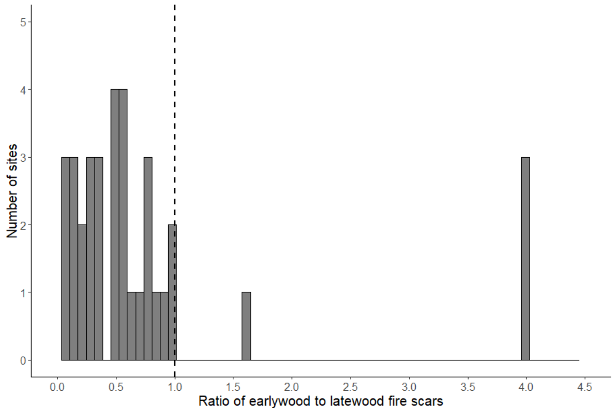
Figure 9—Distribution of site-level values ( n = 39 ) of the proportion of fire scars present in earlywood relative to latewood from seven studies in Colorado ponderosa pine ecosystems. The dashed line at value 1.0 marks the point where observations are equal between seasons; to the left are observations with a majority of latewood fire scars, and to the right are observations with a majority of earlywood fire scars.
