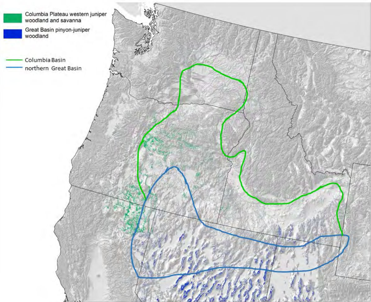
Figure 2—Distribution of juniper communities in the Columbia and northern Great basins based on the LANDFIRE Biophysical Settings (BpS) data layer [84]. LANDFIRE did not map BpSs 0911150, 1710170, and 1811150 because they are uncommon in these regions. Click on the map for a larger image.
