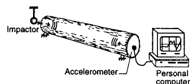
Figure 2. – Experimental test setup.
