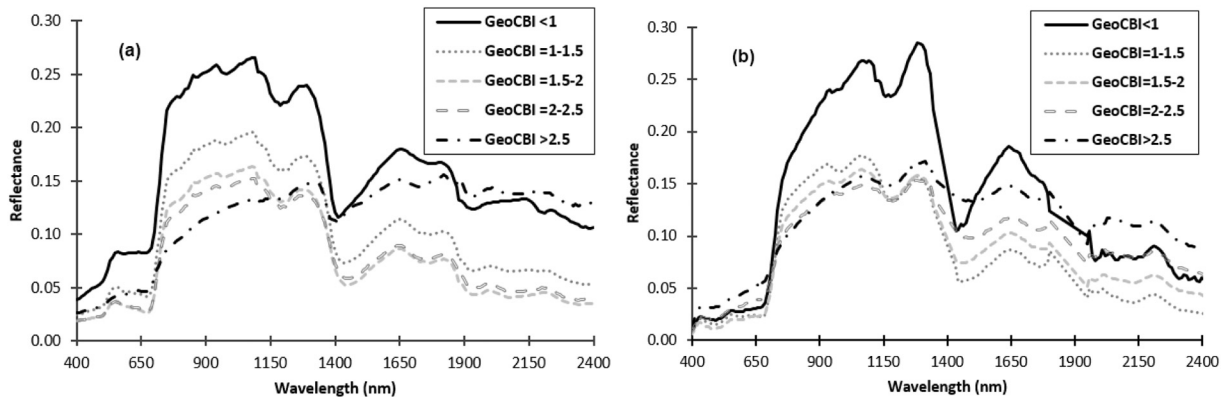
Fig. 3. Average spectral reflectance corresponding to the main intervals of GeoCBI for (a) healthy and (b) diseased trees. Healthy tree spectra were derived from De Santis and Chuvieco (2009).
