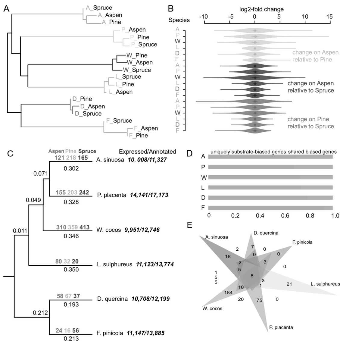
Fig. 1 Patterns of gene expression in response to three different substrates from the six brown rot fungi species. a Neighbor-joining tree with branch length inferred using expression distance (1- Spearman's rho) for all pairs of species. b The fold change of all genes in response to one substrate relative to the other one. c Numbers of substrate-biased genes plotted on the branches of a simplified phylogenetic tree (branch lengths are labeled along the branches). d The proportion of uniquely substrate-biased and shared substrate-biased genes from each species. The two categories are illustrated in Figure S1. e Venn
