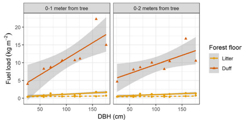
Fig. 3 Scatter plot of the fuel loading of litter and duff ≤1 m from trees (left) and ≤2 m from 830 trees (right), in the Yosemite Forest Dynamics Plot, Yosemite National Park, California, USA, in 2011, before the 2013 Rim Fire. Regression lines are for linear regression (see Additional files 11 and 12 for coefficients). Solid lines show pre-fire fuel loadings, and dashed lines show post-fire total fuel loading. Gray shading shows 95% confidence intervals
