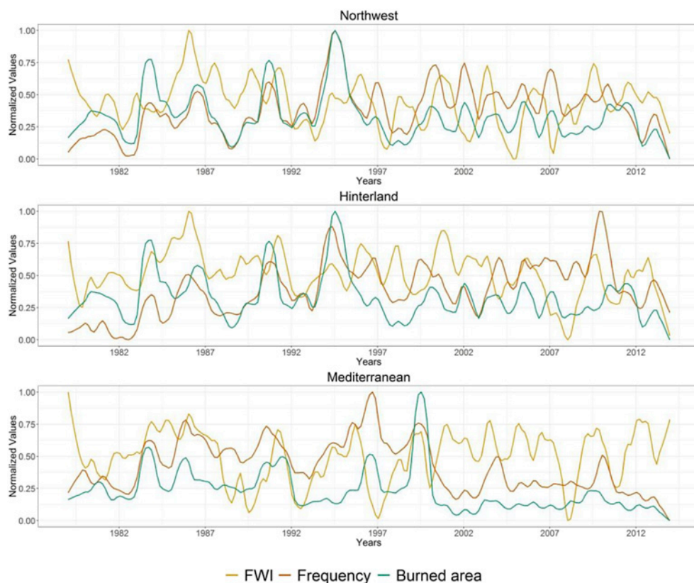
Fig. 6. Time series of trend component of FWI (yellow line), fire frequency (red line) and burned area (green line). All variables are normalized into a 0–1 range. (For interpretation of the references to colour in this figure legend, the reader is referred to the Web version of this article.)
