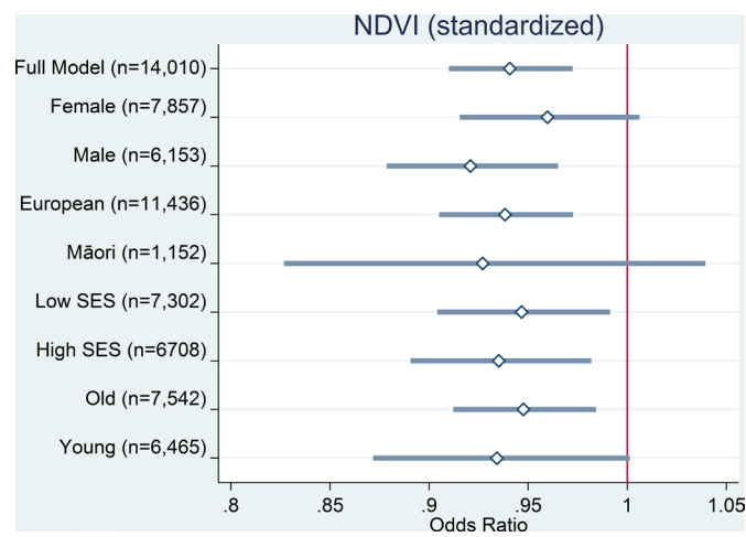
Figure 1 OR plot of standardised mean postsurgical NDVI for time to all-cause mortality following hip or knee arthroplasty (number of participants=14 010, number of observations=149 523). † Low/high SES denotes participants whose lifetime NZ deprivation index is above/below average. Old/young denote participants who are older/younger than the sample mean. The ethnicity reference group is a composite of all ethnicities other than European NZ or Māori (figures 1 and 2 were created with the user-written Stata command COEFLOT). † Following IDI protocols, all sample sizes have been rounded to the nearest multiple of three. IDI, Integrated Data Infrastructure; NDVI, Normalised Difference Vegetation Index; NZ, New Zealand; SES, socioeconomic status.
