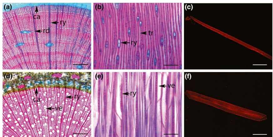
FIGURE 1 Transverse stem sections of a gymnosperm species, Pinus radiata (a) and an angiosperm hybrid, Populus deltoides × Populus nigra (d); scale bars are 200 µm. Tangential stem sections of Pinus radiata (b) and P. deltoides × P. nigra (e); scale bars are 100 µm. Single Pinus radiata tracheid (c) and P. deltoides × P. nigra vessel element (f); scale bars are 100 µm. Cambium (ca); Resin duct (rd); Ray (ry); tracheid (tr)
