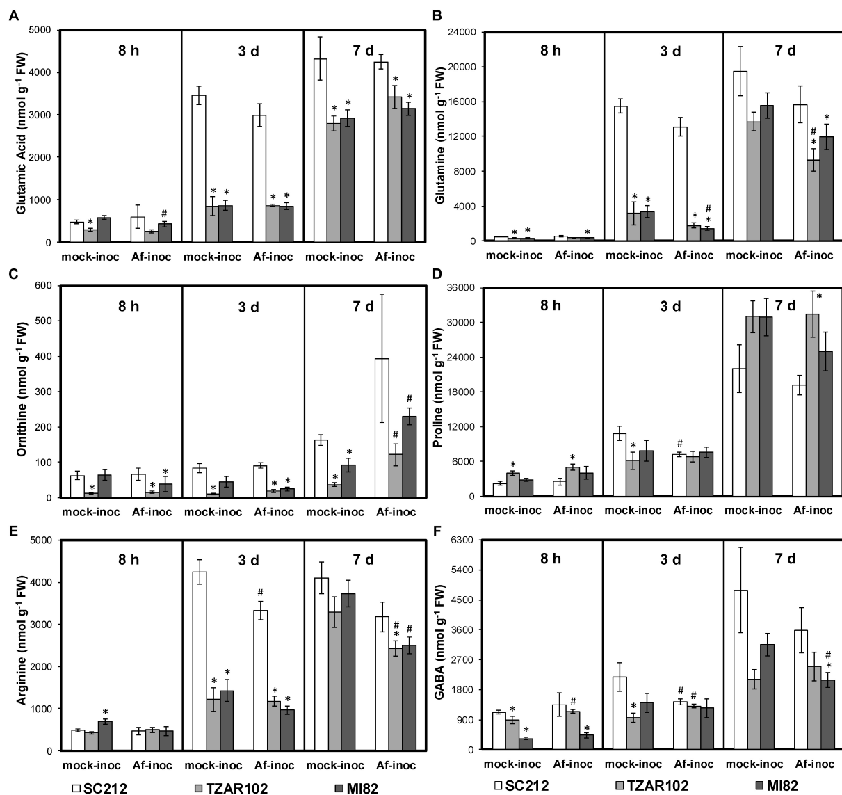
FIGURE 4 | Amino acids are differentially regulated in the susceptible vs. resistant lines. Cellular contents of (A) glutamate, (B) glutamine, (C) ornithine, (D) proline, (E) arginine, and (F) \gamma -aminobutyric acid (GABA) at 8 h, 3 and 7 days in the mock-inoculated (mock-inoc) and A. flavus inoculated (Af-inoc) kernels of susceptible (SC212) and resistant (TZAR102, MI82) maize genotypes. Data are Mean \pm SE of 4 replicates, each replicate consists of six seeds * P \leq 0.05 , between the susceptible line SC212 and other lines; # P \leq 0.05 , between mock and +Af treatments within each line at different times after inoculation).
