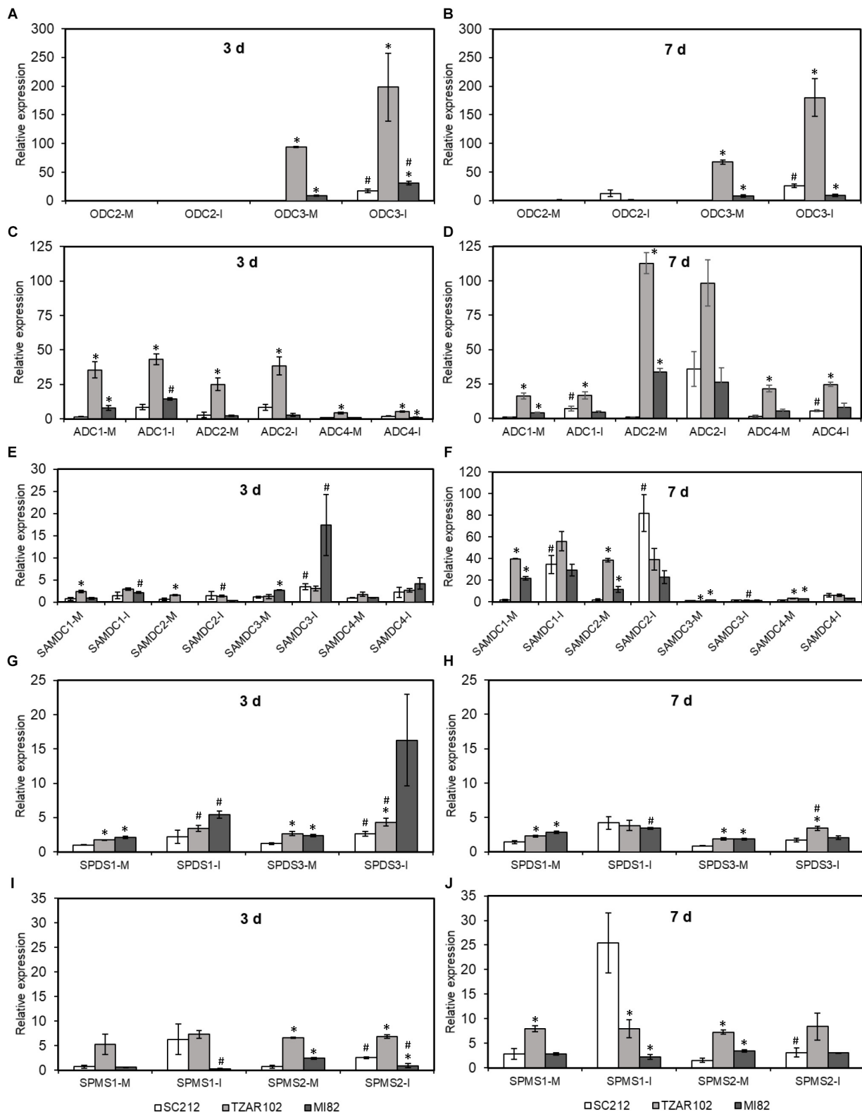
FIGURE 5 | Polyamine biosynthetic genes are highly induced by A. flavus . Expression of maize polyamine biosynthetic genes, (A,B) ODC , (C,D) ADC , (E,F) SAMDC , (G,H) SPDS , (I,J) SPMS at 3 and 7 days in the mock-inoculated (mock-inoc) and A. flavus inoculated (Af-inoc) kernels of susceptible (SC212) and resistant (TZAR102, MI82) maize genotypes. Data are Mean \pm SE of 3 replicates, each replicate consists of six seeds (* P \leq 0.05 , between the susceptible line SC212 and other lines; # P \leq 0.05 , between mock and +Af treatments within each line at different times after inoculation).
