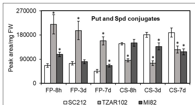
FIGURE 3 | Putrescine and spermidine conjugates detected are differentially affected in the susceptible (SC212) and resistant (TZAR102, MI82) maize genotypes. Cellular contents of N,N' -di-feruloyl-putrescine (FP) and N,N' -di-coumaroyl spermidine (CS) in the A. flavus inoculated kernels at 8 h, 3 and 7 days post-infection. Data are Mean \pm SE of 5 replicates, each replicate consists of six seeds (* P \leq 0.05 , between the susceptible line SC212 and other lines at different times after inoculation).
