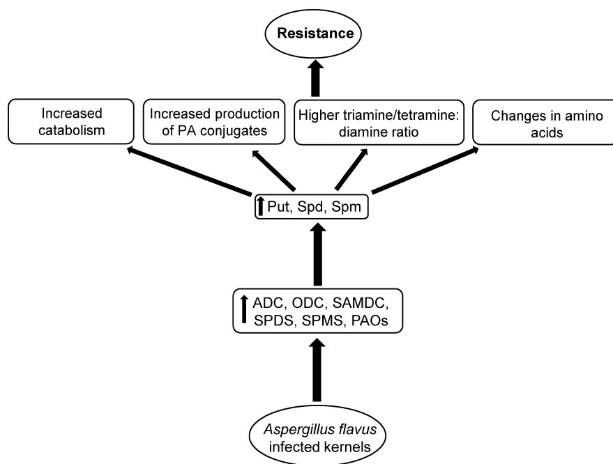
FIGURE 9 | Proposed mechanism of polyamine (PA) mediated A. flavus resistance in maize. Kernel infection of A. flavus resistant maize genotypes results in up-regulation of PA biosynthetic and catabolic genes, and increases cellular PAs. This in turn is followed by increased PA catabolism, production of specific PA conjugates, and specific AAs that might be associated with increased A. flavus resistance and reduced aflatoxin production in the resistant maize genotypes.
