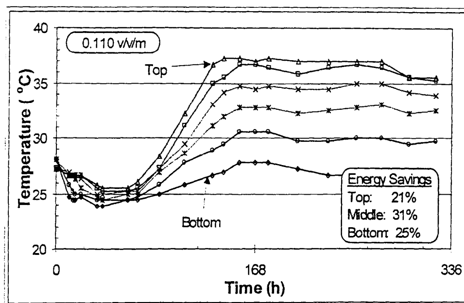
Figure 3. The temperature profiles in a tubular reactor as a function of time. The temperature quickly rises after the third day of incubation indicating a rapid increase in the heat production of the fungus.
