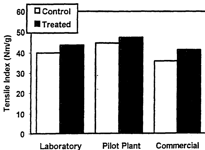
Figure 4. Tensile Index of pulps at different refining scales. All chips were treated in 50-ton outdoor piles.
