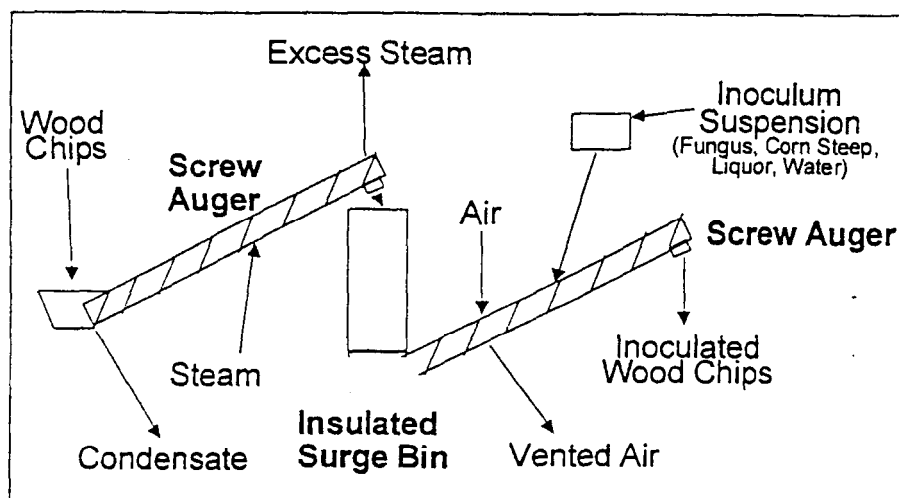
Figure 2. Continuous treatment system to decontaminate, cool, and inoculate wood chips. Wood chips are steamed in the first screw conveyor before being placed into a surge bin. The second screw conveyor then picks up the chips, cools them, and applies the inoculum.
