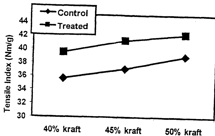
Figure 5. Tensile Index of TMP pulps blended with different levels of bleached softwood kraft pulp.
