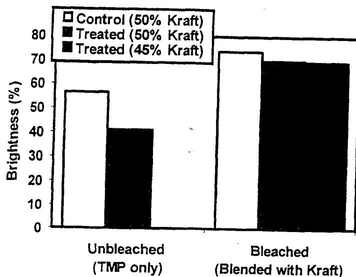
Figure 7. Brightness of unbleached and bleached and blended TMP pulps.
