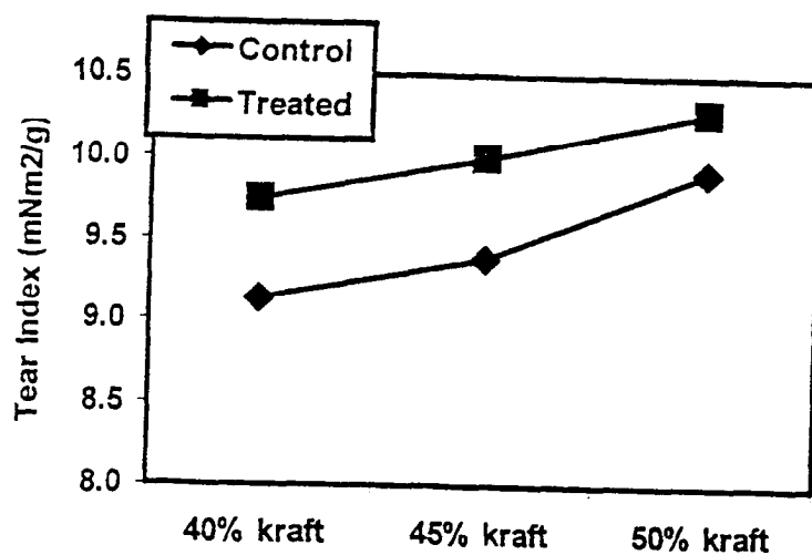
Figure 6. Tear Index of TMP pulps blended with different levels of bleached softwood kraft pulp.
