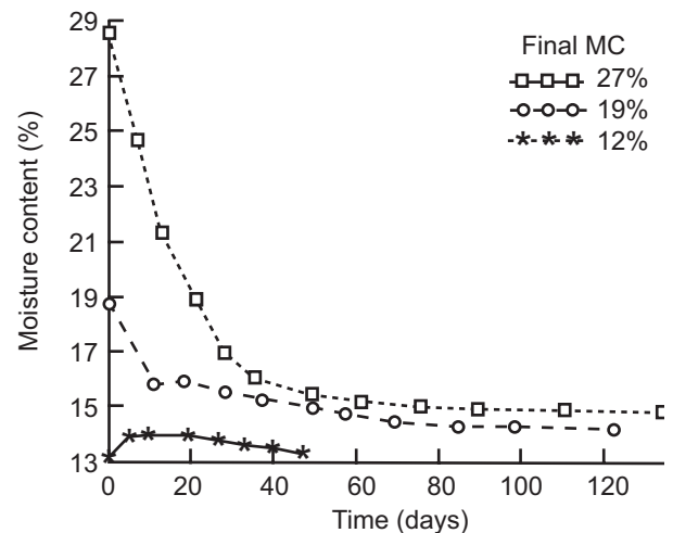
Figure 2—Curves showing moisture content loss during equilibration of sugar maple 2 by 6's.
