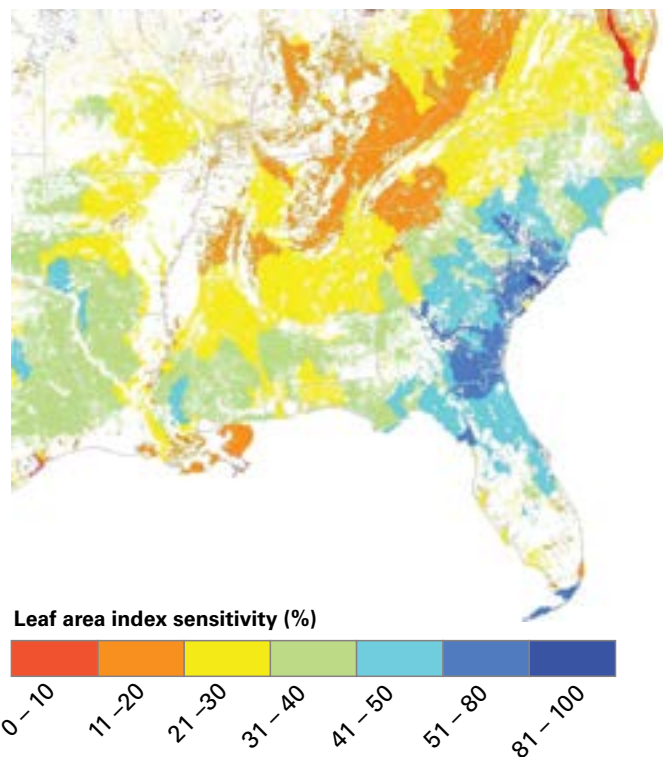
Figure 9.13—Water yield response to 50-percent reduction of leaf area index as simulated by the Water Supply Stress Index model. (Source: Sun et al. 2015a)
