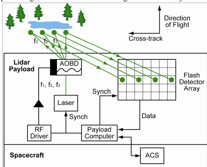
Figure 1. A schematic of the Electronically Steerable Flash Lidar concept.
