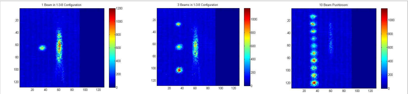
Figure 2. The image of the scattering form the ground of three sequential laser pulses taken form an aircraft. ESFL has been commanded to change the number of beamlets for each laser pulse. Along track direction is left to right. Elongated beam is the undeflected beam which has been optically reshaped and re-aligned to fall ahead of the deflected beams.
