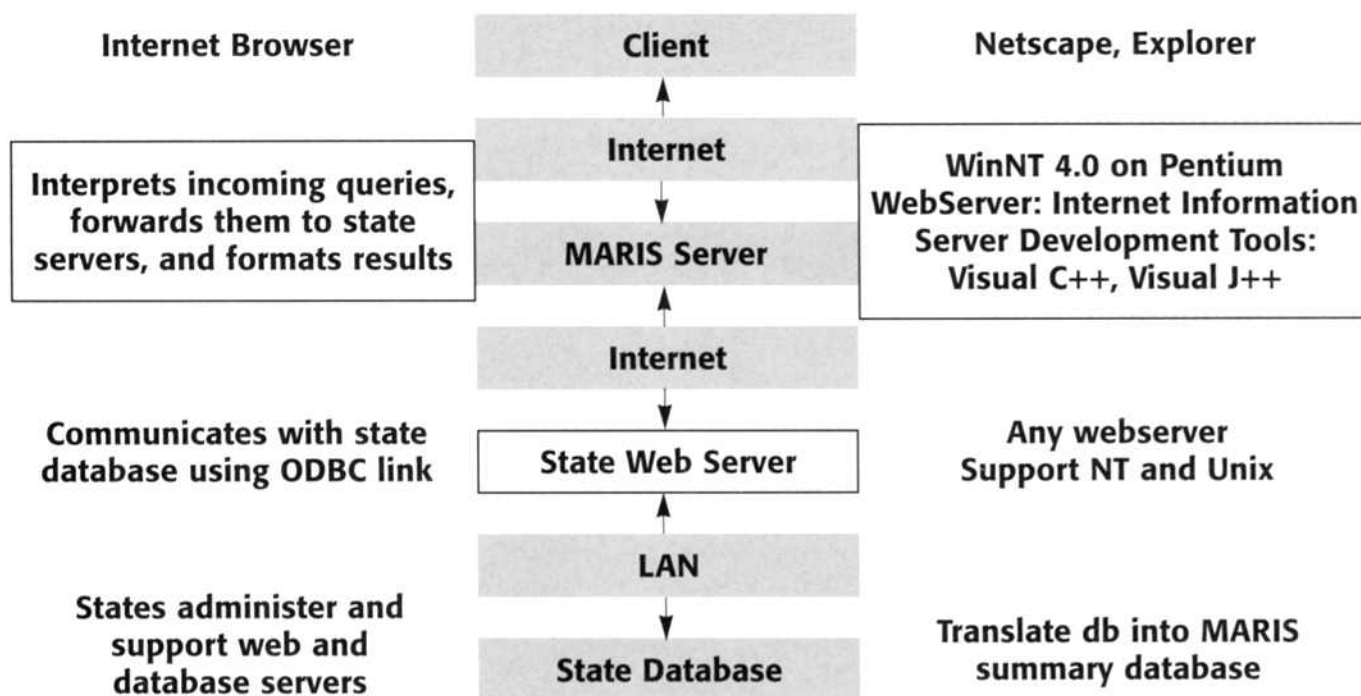
Figure 1 shows the method by which the Multi-state Aquatic Resources Information System collects data from state World Wide Web servers received from end users wanting access to these data.
