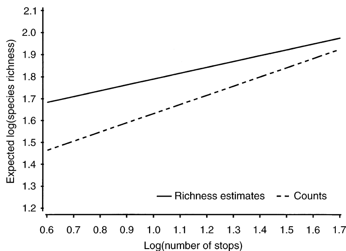
FIG 1. Species–area relationships based on count data and estimates of species richness [model M(h) ] from 51 BBS routes in Maryland, USA. Expected values are based on a linear model. The model fitted is Y = \beta X + \alpha , where Y = \log_{10}(\text{species richness}) and X = \log_{10}(\text{number of units of area}) .
