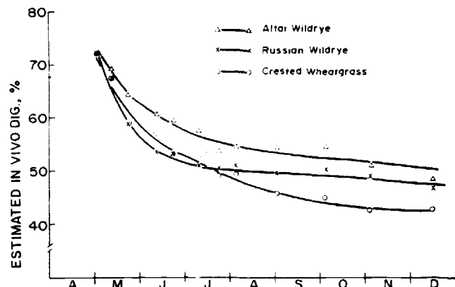
Figure 15.--Estimated in vivo digestibility of three grasses grown at Sidney, Montana (adapted from White and Wight 1981).
