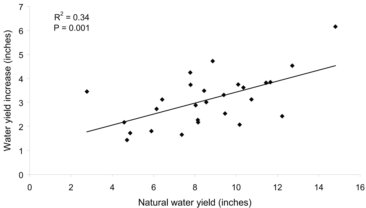
Figure 2.5. Harvest-induced increases in water yield from Fool Creek versus the predicted natural water yield in the absence of any forest harvest. Data are from 1956-1982.
