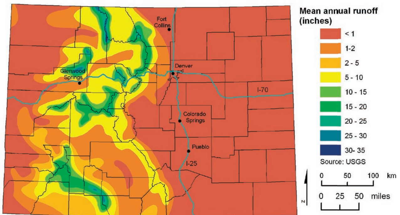
Figure 1.3. Map of mean annual runoff in Colorado.
