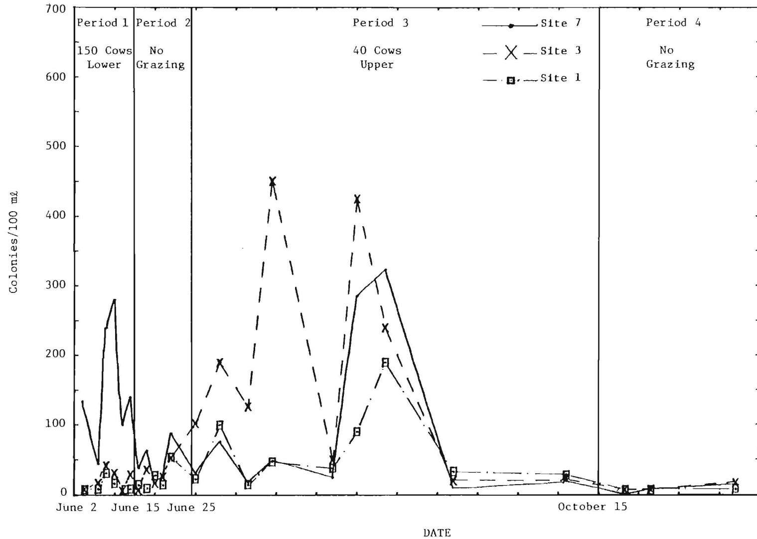
Figure 13. Fecal Coliform Concentrations at Sites 1, 3 and 7 for Periods 1 through 4, 1977.
