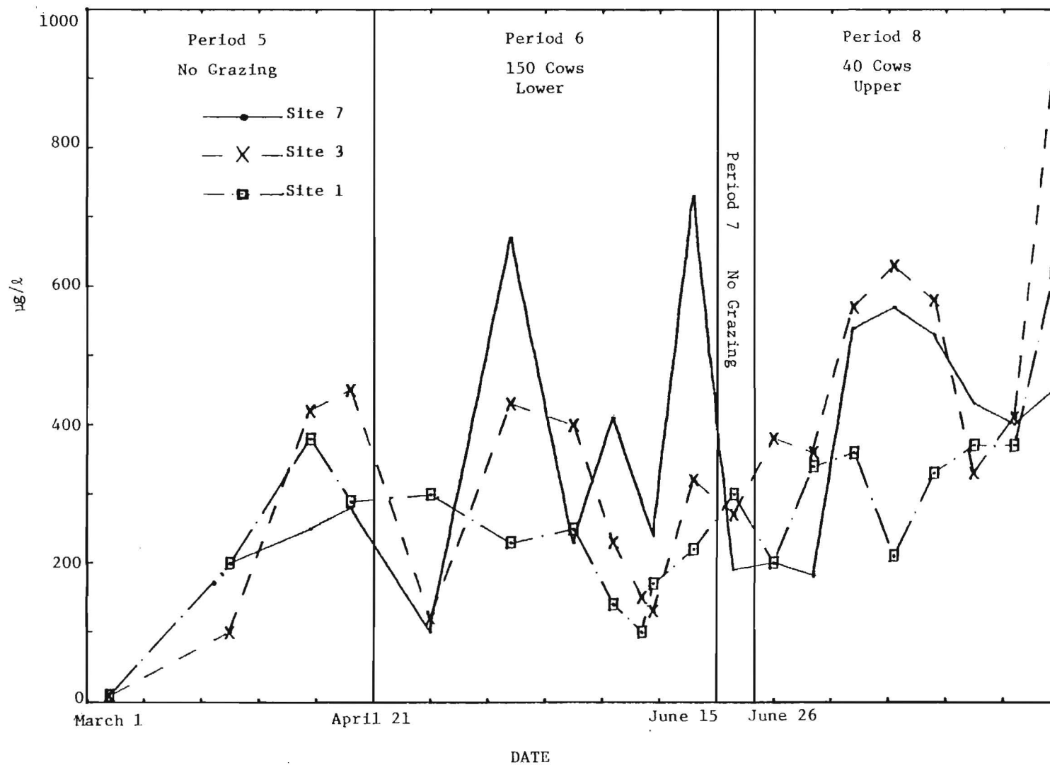
Figure 17. Nitrate-Nitrogen Concentrations at Sites 1, 3 and 7 for Periods 5 through 8, 1978.
