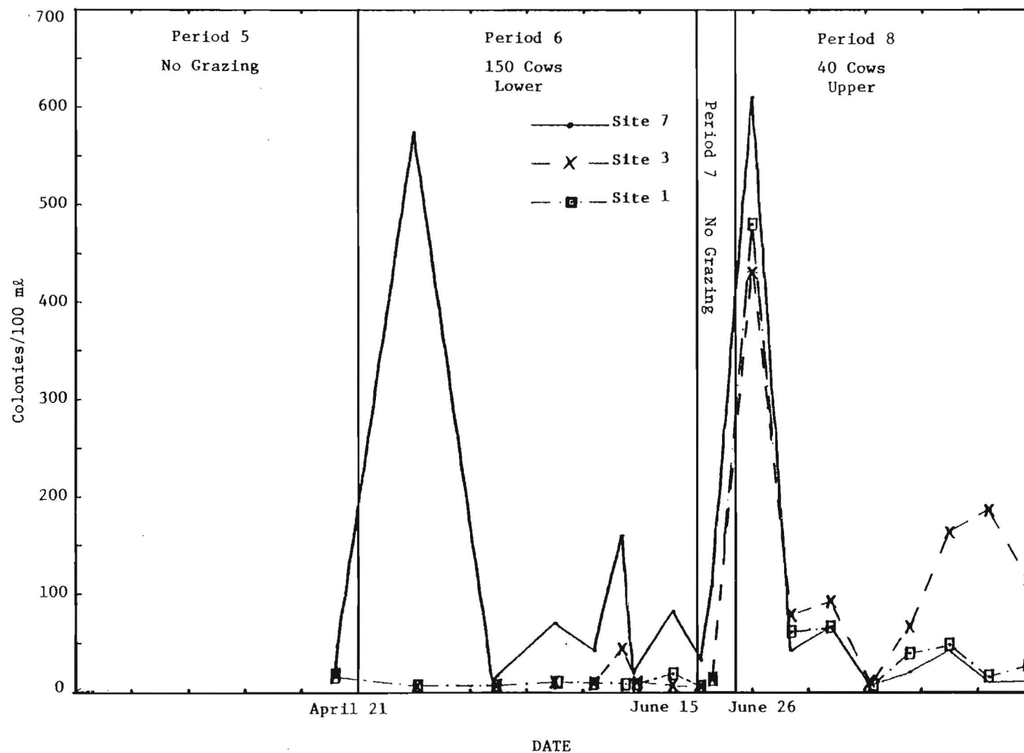
Figure 18. Fecal Coliform Concentrations at Sites 1, 3 and 7 for Periods 5 through 8, 1978.
