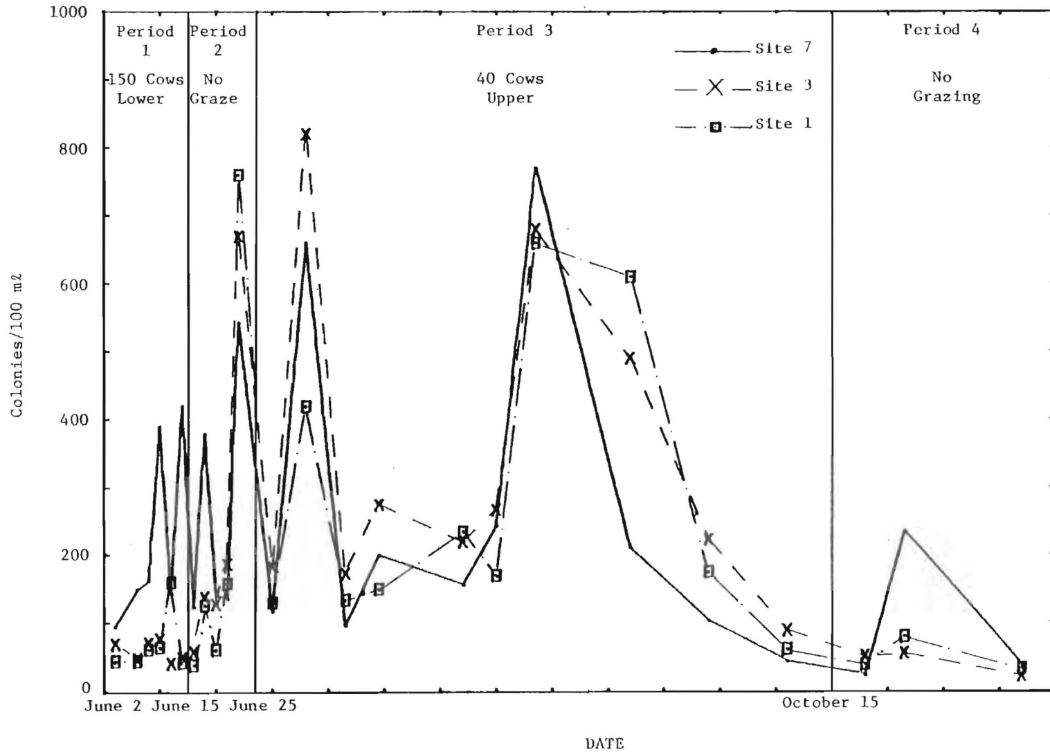
Figure 14. Fecal Streptococci Concentrations at Sites 1, 3 and 7 for Periods 1 through 4, 1977.
