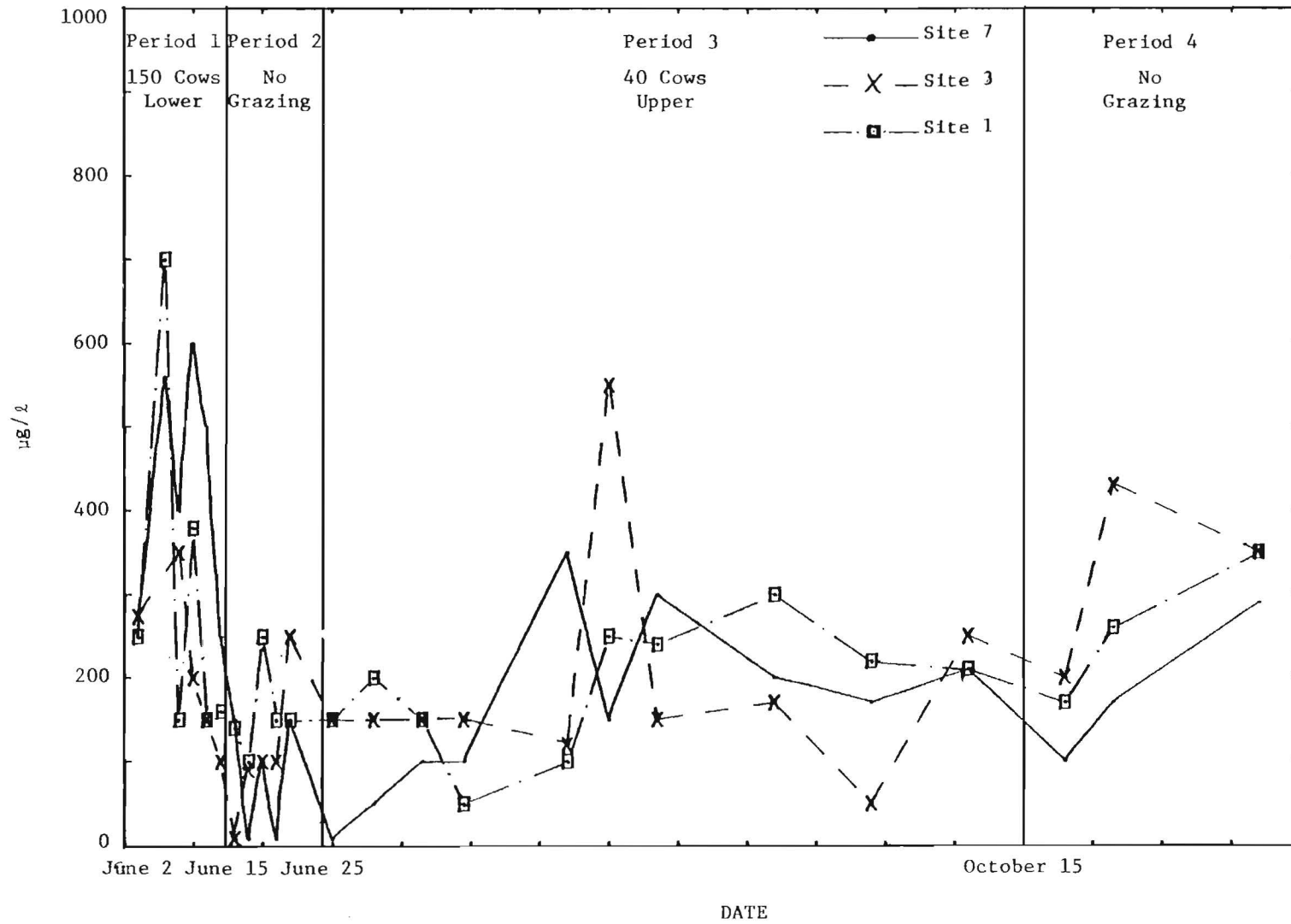
Figure 12. Nitrate-Nitrogen Concentrations at Sites 1, 3 and 7 for Periods 1 through 4, 1977.
