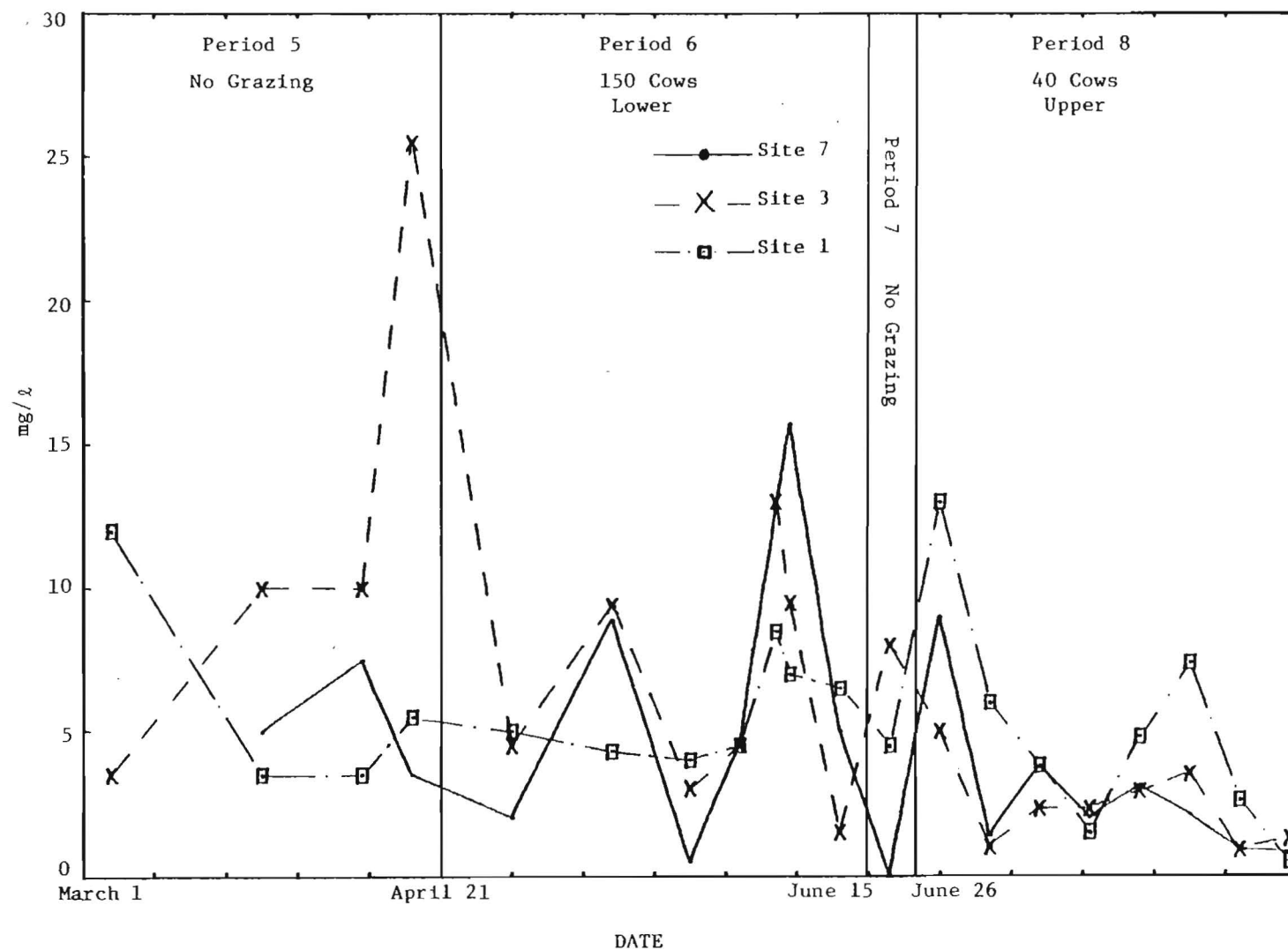
Figure 15. Suspended Solids Concentrations at Sites 1, 3 and 7 for Periods 5 through 8, 1978.
