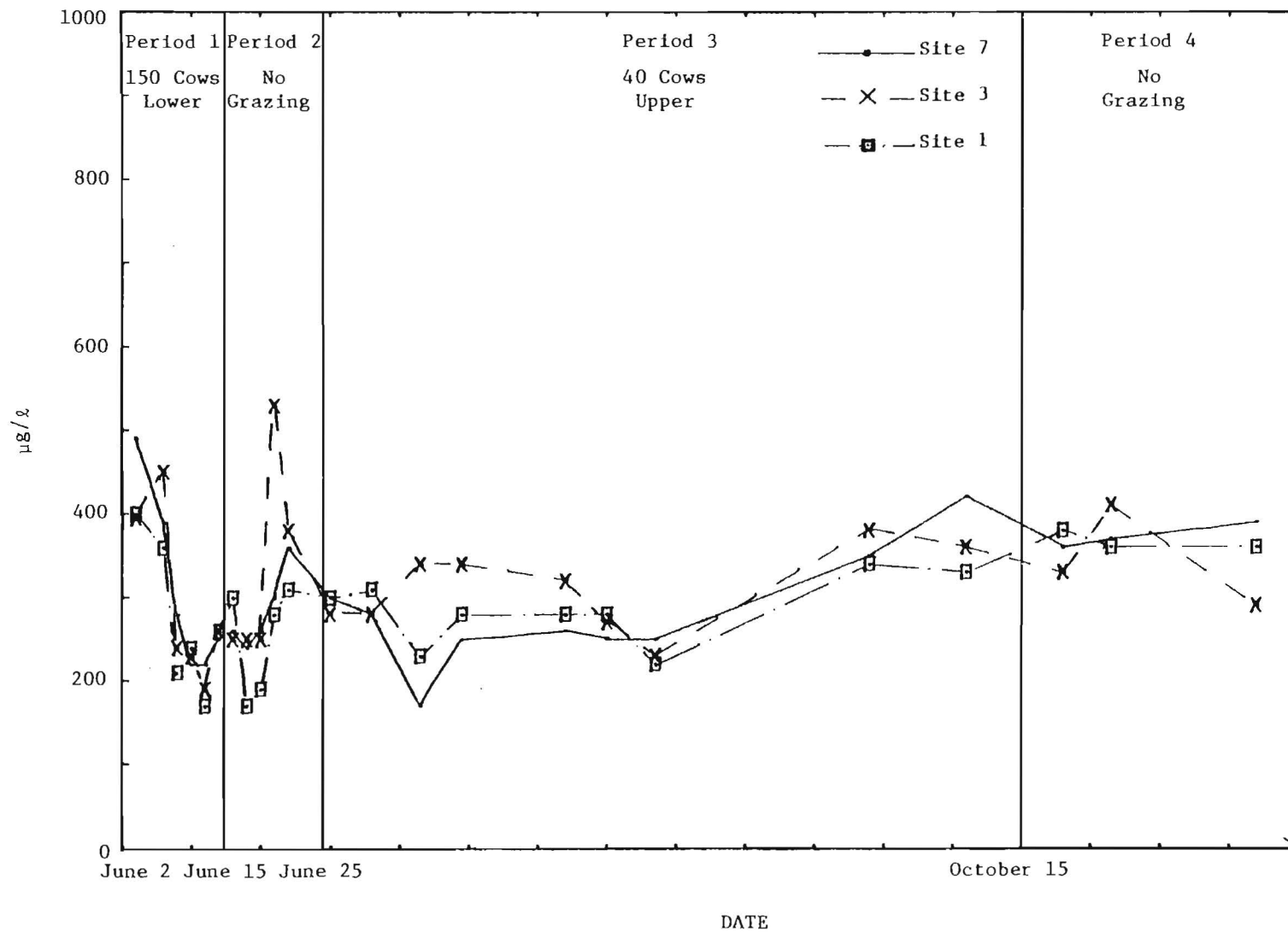
Figure 11. Ammonia-Nitrogen Concentrations at Sites 1, 3 and 7 for Periods 1 through 4, 1977.
