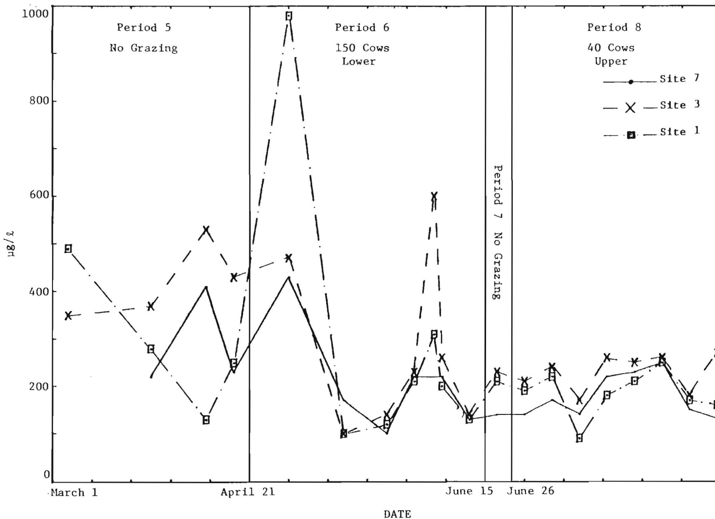
Figure 16. Ammonia-Nitrogen Concentrations at Sites 1, 3 and 7 for Periods 5 through 8, 1978.
