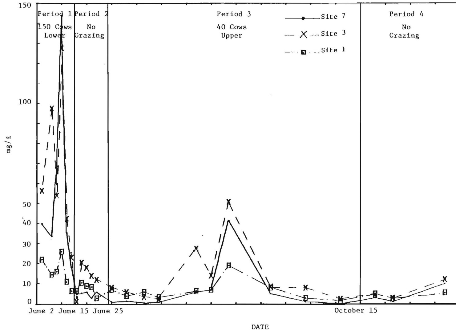
Figure 10. Suspended Solids Concentrations at Sites 1, 3 and 7 for Periods 1 through 4, 1977.
