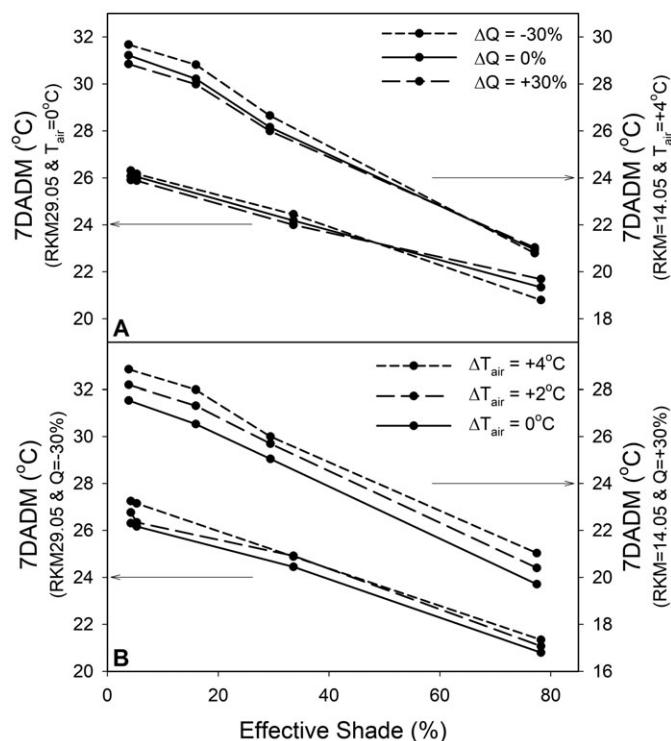
FIGURE 7. Interactive effects of either (a) stream discharge or (b) air temperature with shade. (a) Left y-axis shows RKM29.05 with T_{\text{air}} = 0^{\circ}\text{C} ; right y-axis shows RKM14.05 with T_{\text{air}} = +4^{\circ}\text{C} . (b) Left y-axis shows RKM29.05 with -30\% Q ; right y-axis shows RKM14.05 with +30\% Q . Note that the y-axes are offset by several degrees, as indicated by thin horizontal arrows pointing to 24^{\circ}\text{C} , to keep lines from overlapping and making the graph difficult to read.
