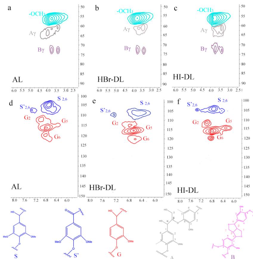
Figure 4. HSQC spectra of AL and DL samples: Signals for sidechain in (a) AL (b) HBr-DL (c) HI-DL and signals for aromatic ring in: (d) AL (e) HBr-DL (f) HI-DL. Assignments for ^{13}\text{C} - ^1\text{H} cross-signals provided in Table 3.
