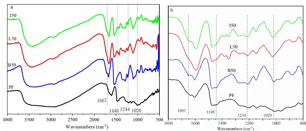
Figure 5. (a) FT-IR spectra of PF, ALPF (L50), and DLPF (I50, B50) resins with 50% lignin substitution; (b) enlarged spectral region shows signals of particular interest.
