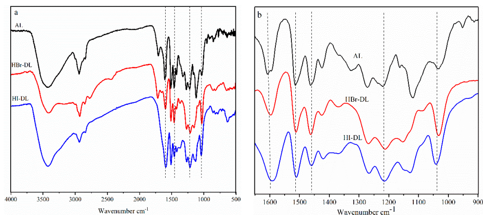
Figure 2. (a) FT-IR spectra of alkali lignin (AL) and demethylated lignins (DL) with HBr or HI as the reagent; (b) enlarged spectral region shows signals of particular interest.
