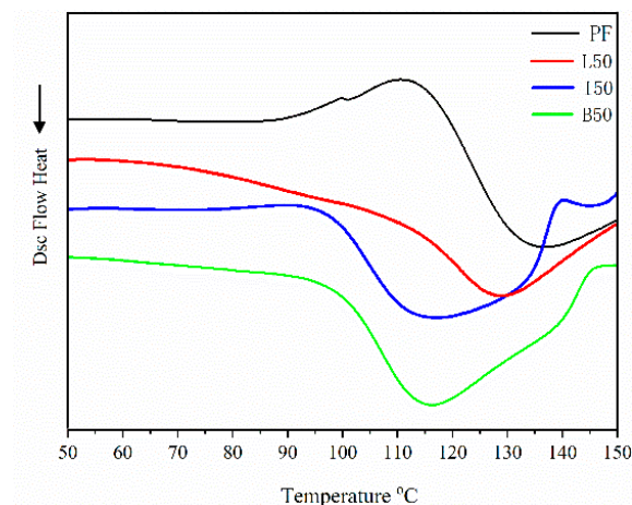
Figure 7. DSC analysis of PF, ALPF(L50), DLPF (I50, B50) resins with 50% lignin substitution.
