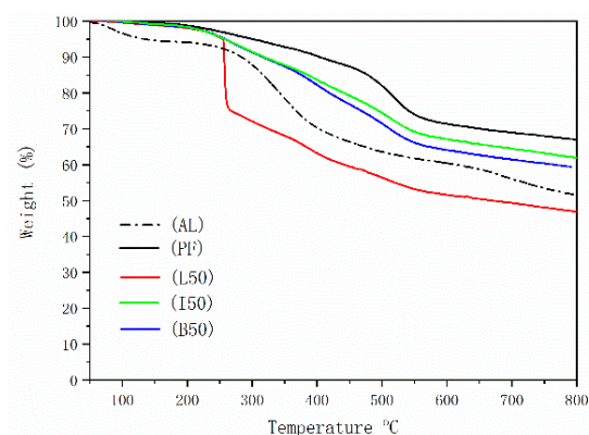
Figure 8. TGA analysis of Alkali lignin, PF, ALPF(L50), DLPF (I50, B50) resins with 50% lignin substitution.
