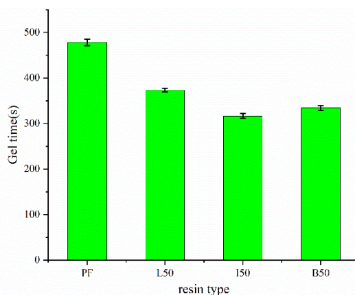
Figure 9. Gel time of PF, ALPF (L50), and DLPF (I50, B50) resins with 50% lignin substitution.
