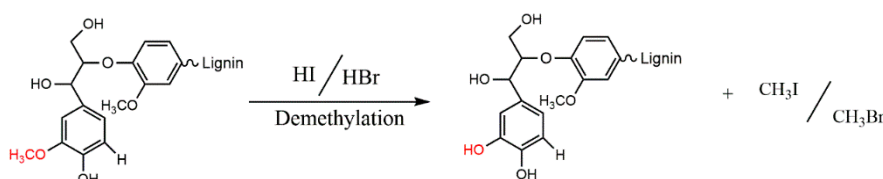
Figure 1. Schematic reaction process of the demethylation of lignin with halogen acids.
