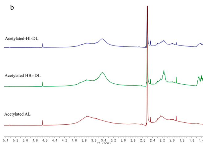
Figure 3. ^1\text{H} -NMR spectra of (a) acetylated AL and demethylated lignins (DL); and (b) enlarged area of the methoxy and acetoxy group.
