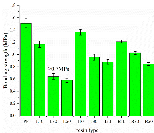
Figure 10. Bonding strength of PF, ALPF, DLPF resins at different lignin substitutions.
