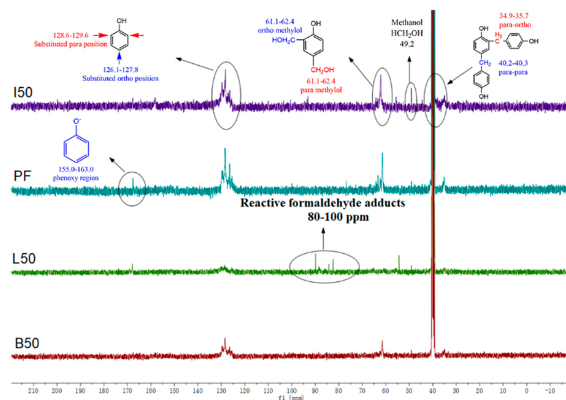
Figure 6. ^{13}\text{C} -NMR spectra of PF, ALPF(L50), and DLPF (I50, B50) resins with 50% lignin substitution.
